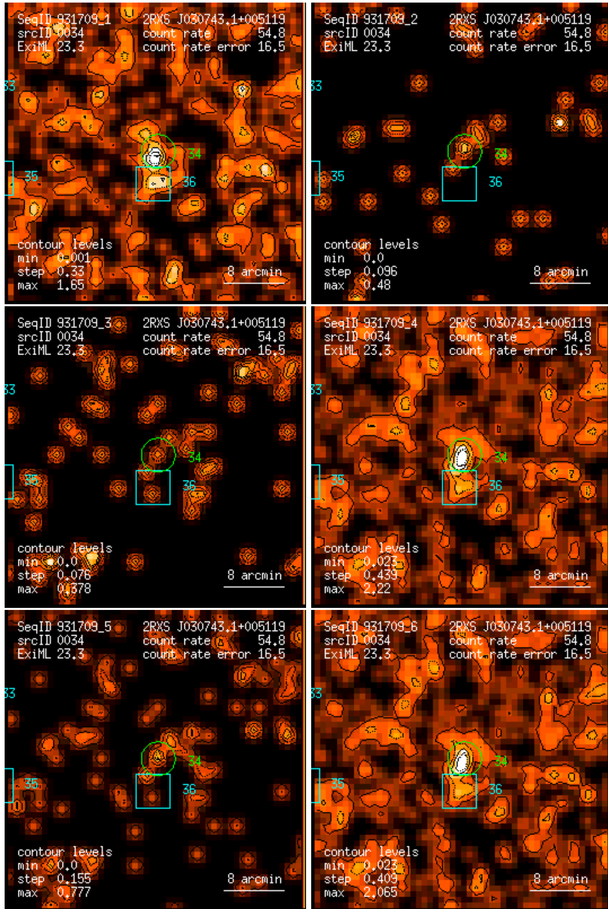
Figure 34: RASS 931709: detection 0034: band rate images, Gaussian filter: (1) PSPC channels 11 – 41, (2) 52 – 90, (3) 91 – 201, (4) 11 – 235, (5) 52 – 201, (6) 11 – 201. Broad band rates in counts/ks. Band rate contour levels in counts/ks/arcmin 2 .
