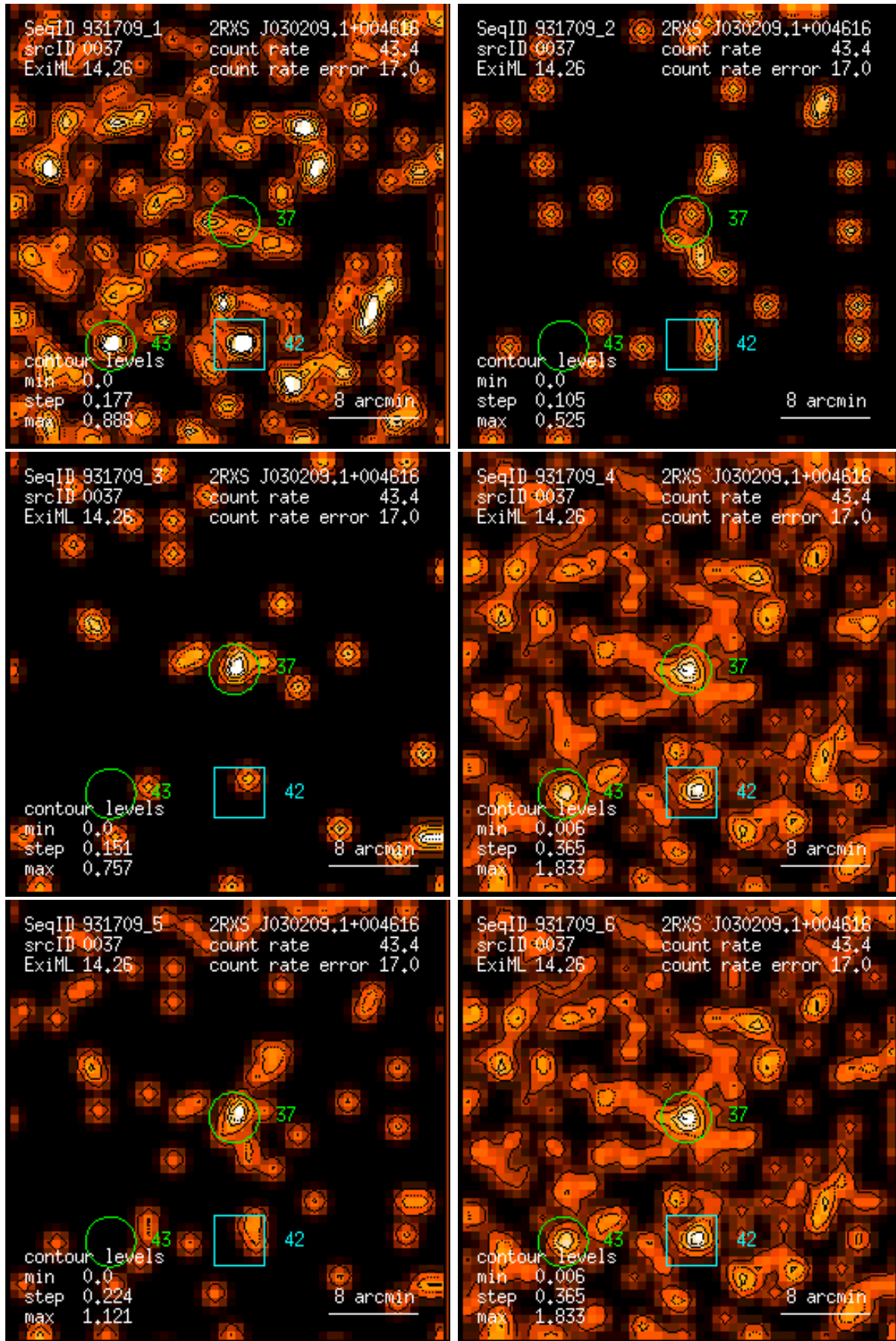
Figure 37: RASS 931709: detection 0037: band rate images, Gaussian filter: (1) PSPC channels 11 – 41, (2) 52 – 90, (3) 91 – 201, (4) 11 – 235, (5) 52 – 201, (6) 11 – 201. Broad band rates in counts/ks. Band rate contour levels in counts/ks/arcmin 2 .
