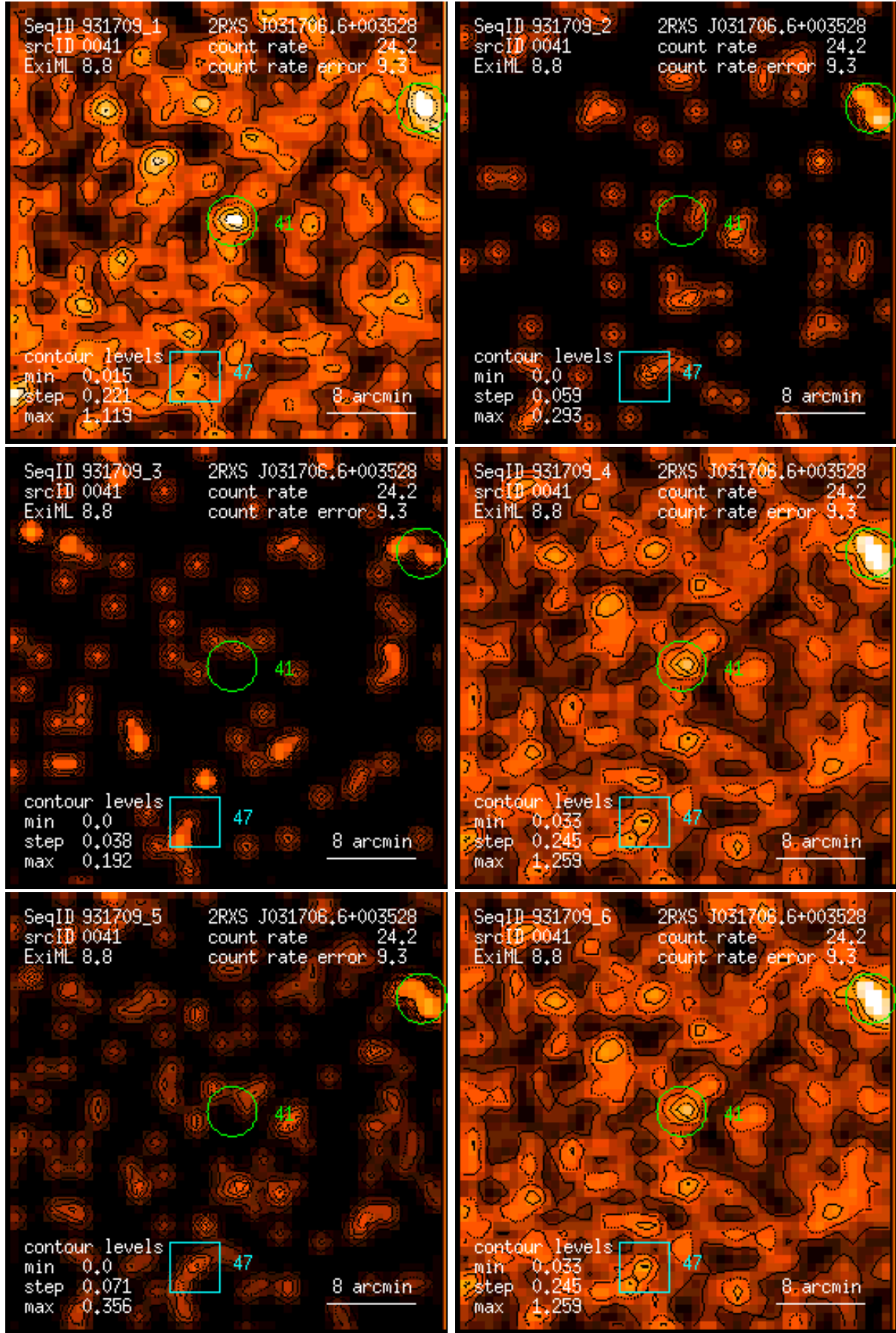
Figure 41: RASS 931709: detection 0041: band rate images, Gaussian filter: (1) PSPC channels 11 – 41, (2) 52 – 90, (3) 91 – 201, (4) 11 – 235, (5) 52 – 201, (6) 11 – 201. Broad band rates in counts/ks. Band rate contour levels in counts/ks/arcmin 2 .
