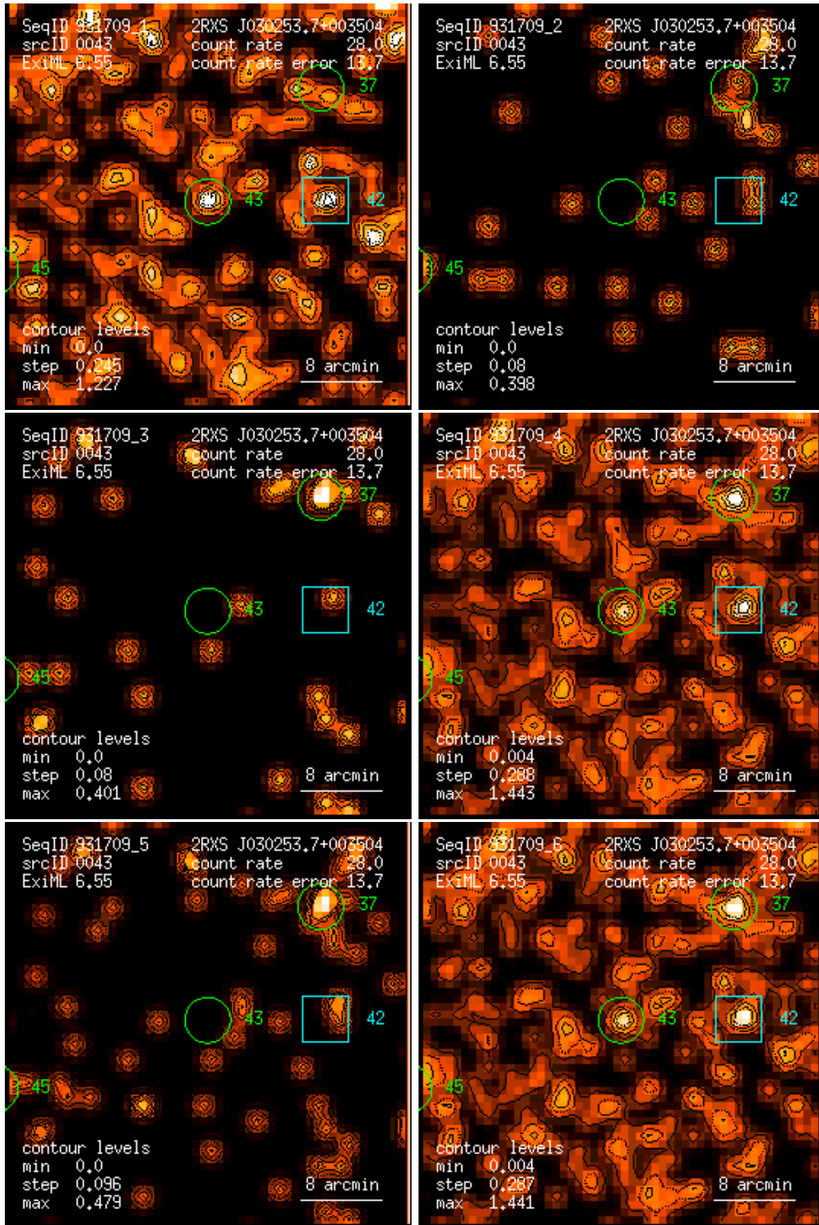
Figure 43: RASS 931709: detection 0043: band rate images, Gaussian filter: (1) PSPC channels 11 – 41, (2) 52 – 90, (3) 91 – 201, (4) 11 – 235, (5) 52 – 201, (6) 11 – 201. Broad band rates in counts/ks. Band rate contour levels in counts/ks/arcmin 2 .
