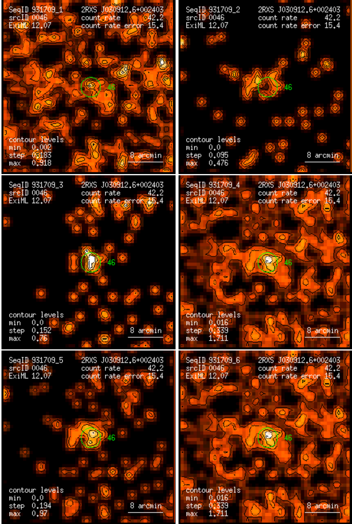
Figure 46: RASS 931709: detection 0046: band rate images, Gaussian filter: (1) PSPC channels 11 – 41, (2) 52 – 90, (3) 91 – 201, (4) 11 – 235, (5) 52 – 201, (6) 11 – 201. Broad band rates in counts/ks. Band rate contour levels in counts/ks/arcmin 2 .
