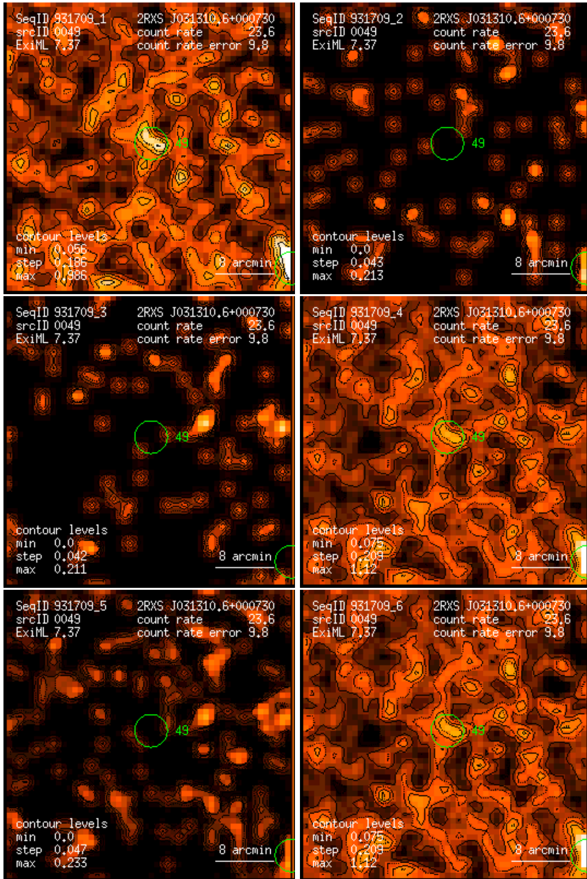
Figure 49: RASS 931709: detection 0049: band rate images, Gaussian filter: (1) PSPC channels 11 – 41, (2) 52 – 90, (3) 91 – 201, (4) 11 – 235, (5) 52 – 201, (6) 11 – 201. Broad band rates in counts/ks. Band rate contour levels in counts/ks/arcmin 2 .
