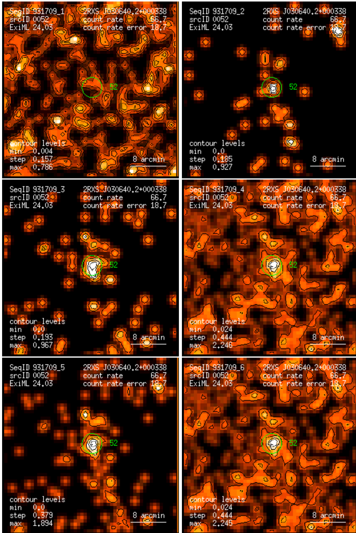
Figure 52: RASS 931709: detection 0052: band rate images, Gaussian filter: (1) PSPC channels 11 – 41, (2) 52 – 90, (3) 91 – 201, (4) 11 – 235, (5) 52 – 201, (6) 11 – 201. Broad band rates in counts/ks. Band rate contour levels in counts/ks/arcmin 2 .
