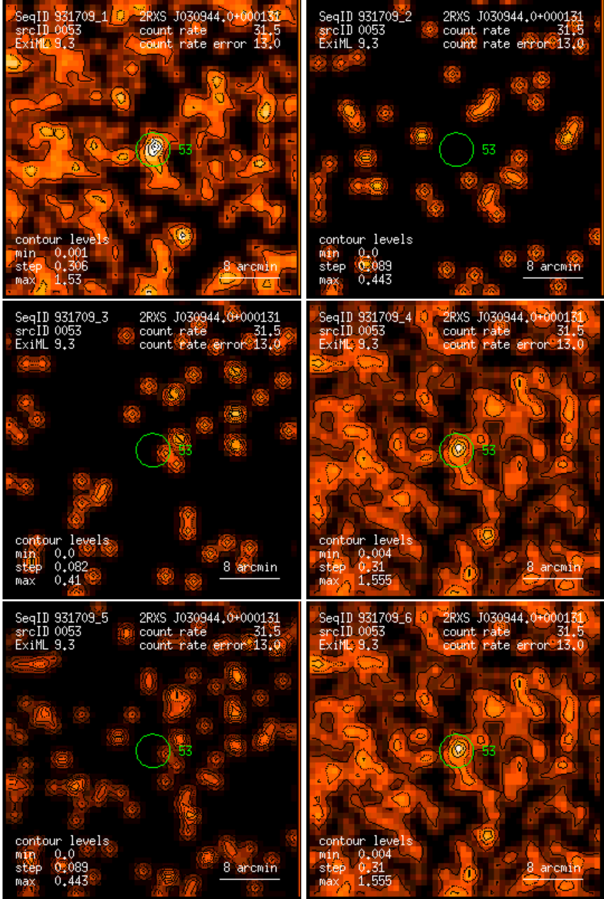
Figure 53: RASS 931709: detection 0053: band rate images, Gaussian filter: (1) PSPC channels 11 – 41, (2) 52 – 90, (3) 91 – 201, (4) 11 – 235, (5) 52 – 201, (6) 11 – 201. Broad band rates in counts/ks. Band rate contour levels in counts/ks/arcmin 2 .
