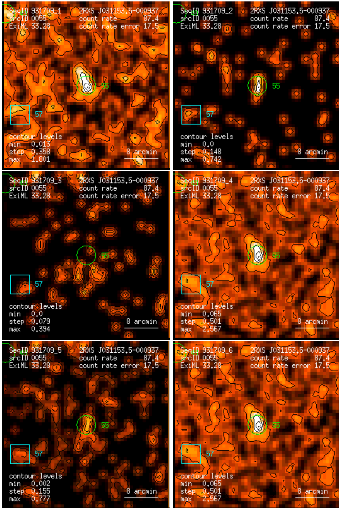
Figure 55: RASS 931709: detection 0055: band rate images, Gaussian filter: (1) PSPC channels 11 – 41, (2) 52 – 90, (3) 91 – 201, (4) 11 – 235, (5) 52 – 201, (6) 11 – 201. Broad band rates in counts/ks. Band rate contour levels in counts/ks/arcmin 2 .
