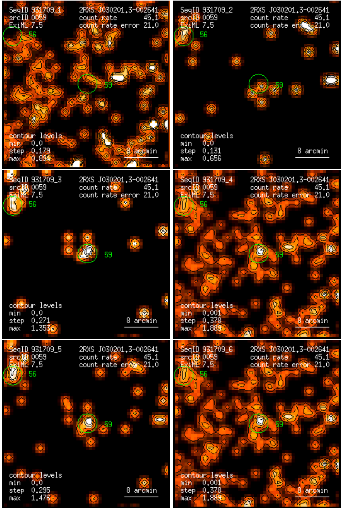
Figure 59: RASS 931709: detection 0059: band rate images, Gaussian filter: (1) PSPC channels 11 – 41, (2) 52 – 90, (3) 91 – 201, (4) 11 – 235, (5) 52 – 201, (6) 11 – 201. Broad band rates in counts/ks. Band rate contour levels in counts/ks/arcmin 2 .
