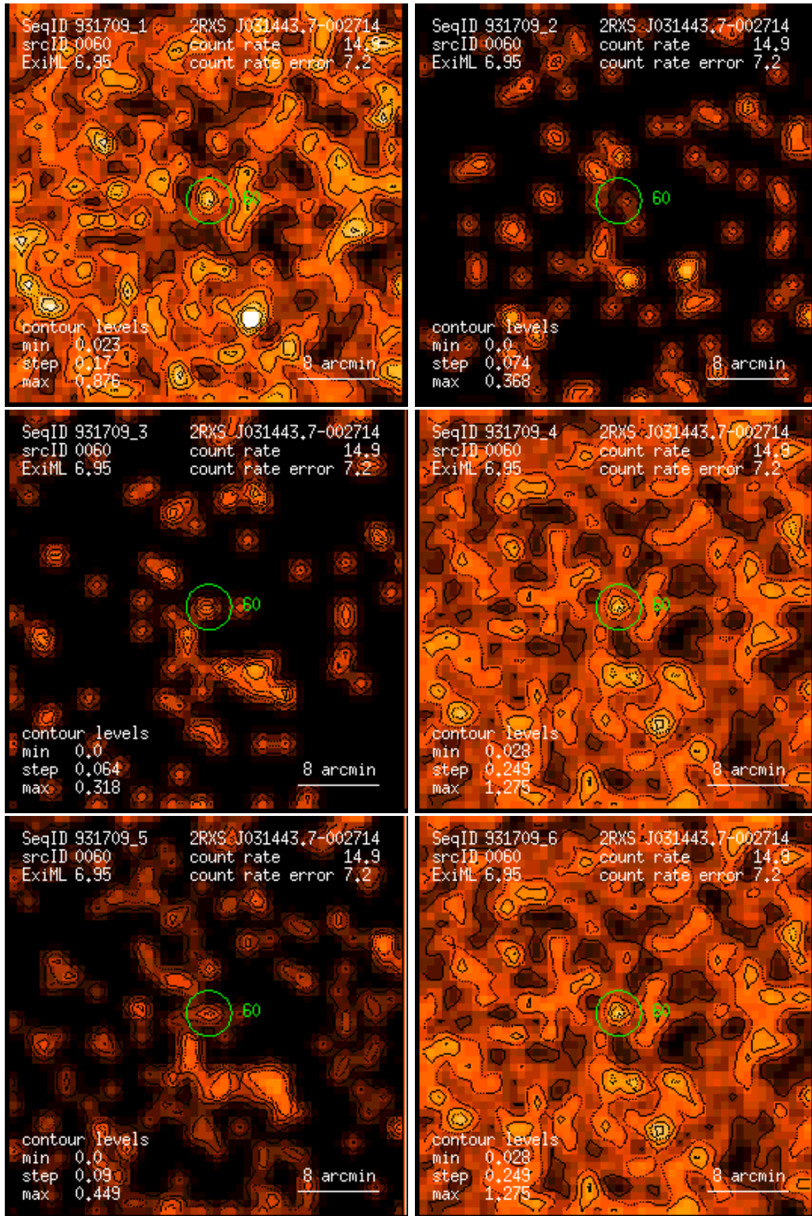
Figure 60: RASS 931709: detection 0060: band rate images, Gaussian filter: (1) PSPC channels 11 – 41, (2) 52 – 90, (3) 91 – 201, (4) 11 – 235, (5) 52 – 201, (6) 11 – 201. Broad band rates in counts/ks. Band rate contour levels in counts/ks/arcmin 2 .
