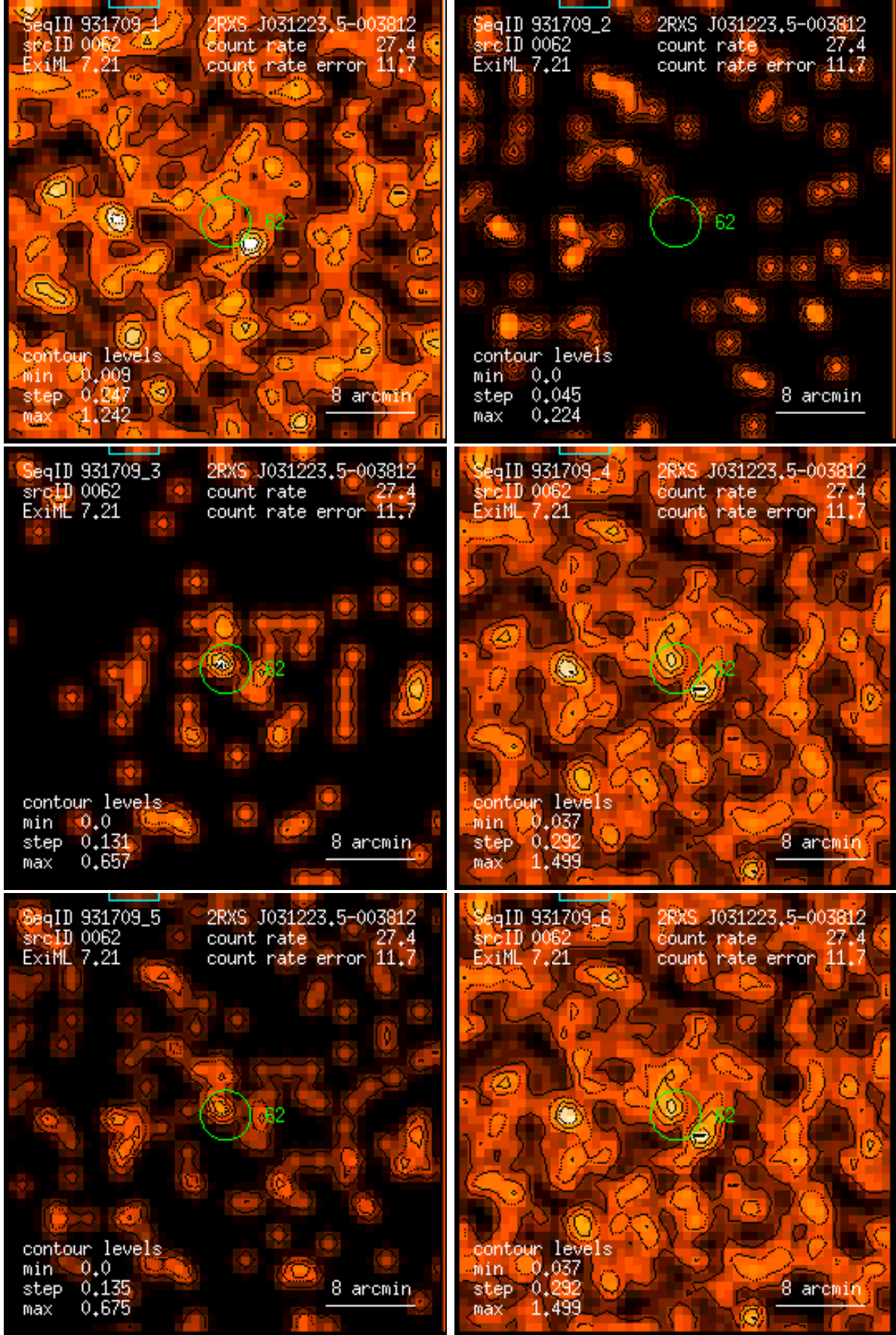
Figure 62: RASS 931709: detection 0062: band rate images, Gaussian filter: (1) PSPC channels 11 – 41, (2) 52 – 90, (3) 91 – 201, (4) 11 – 235, (5) 52 – 201, (6) 11 – 201. Broad band rates in counts/ks. Band rate contour levels in counts/ks/arcmin 2 .
