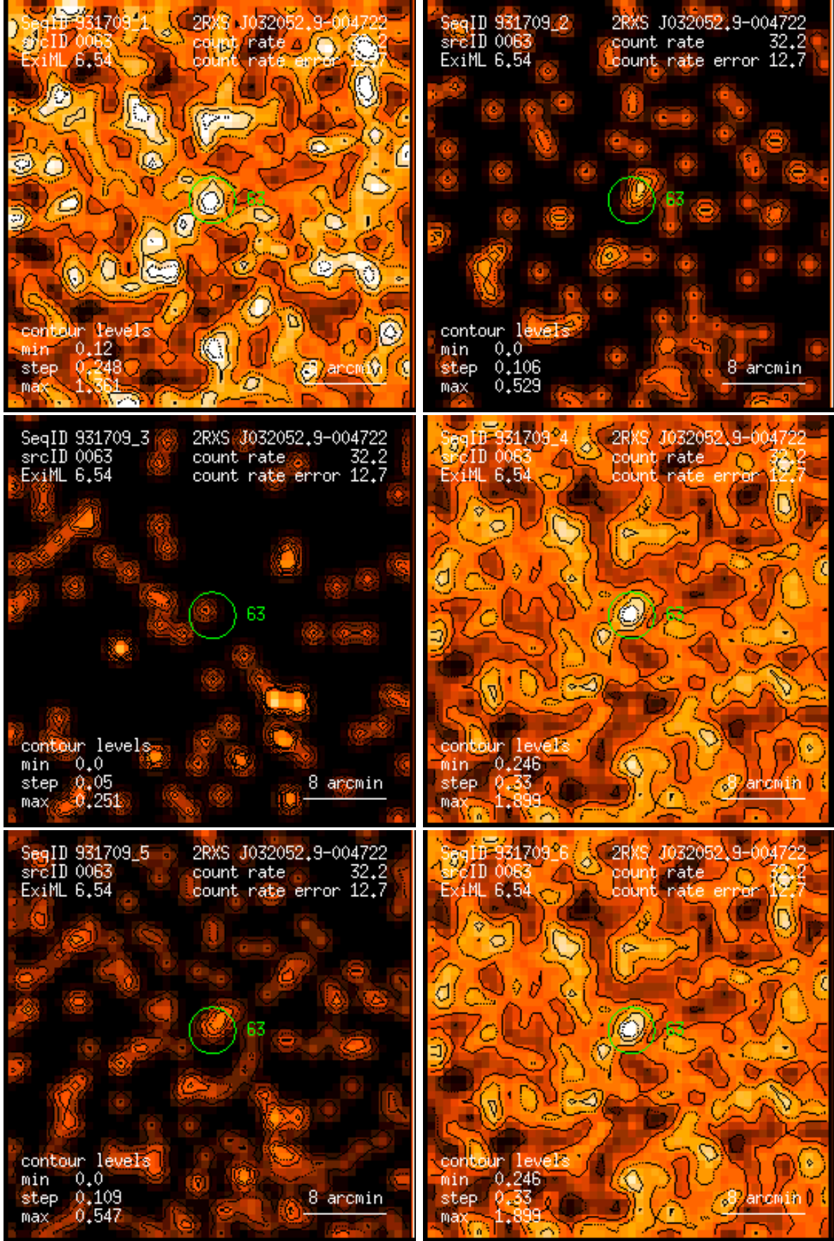
Figure 63: RASS 931709: detection 0063: band rate images, Gaussian filter: (1) PSPC channels 11 – 41, (2) 52 – 90, (3) 91 – 201, (4) 11 – 235, (5) 52 – 201, (6) 11 – 201. Broad band rates in counts/ks. Band rate contour levels in counts/ks/arcmin 2 .
