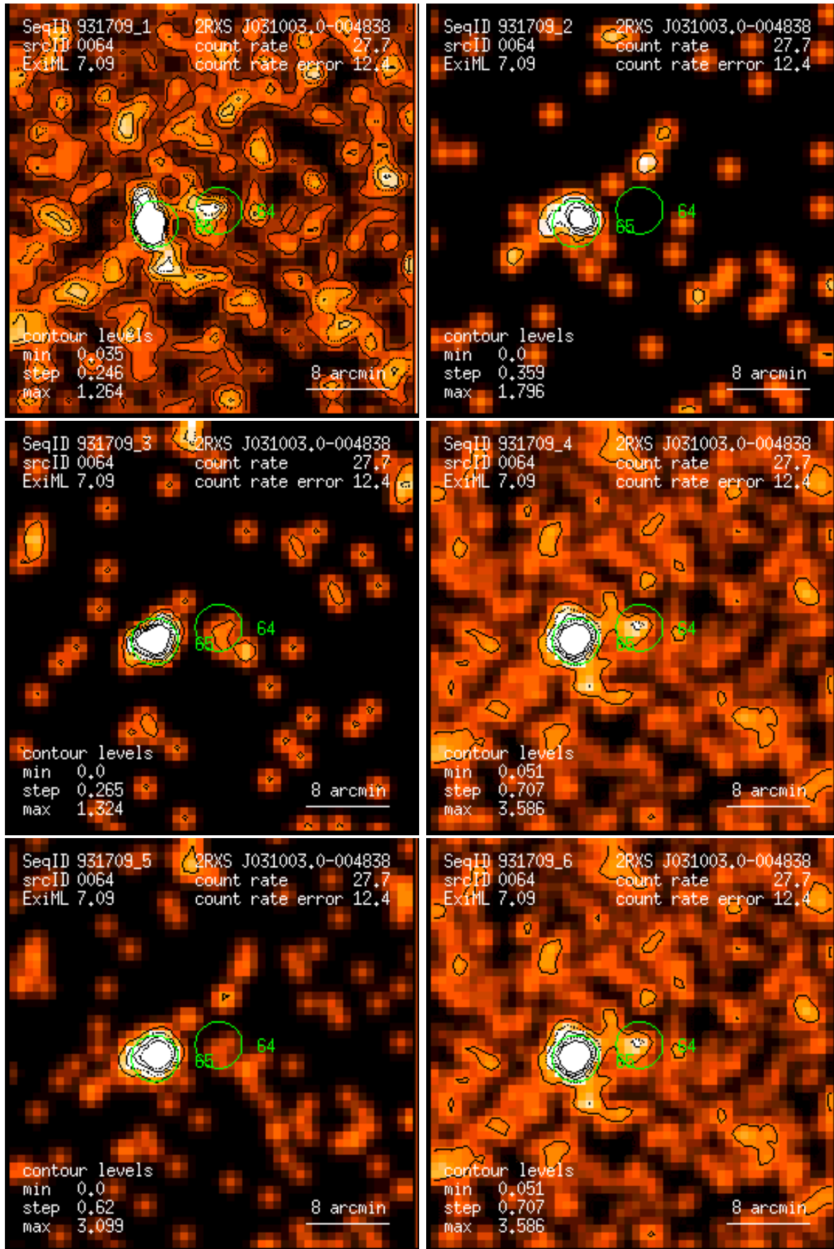
Figure 64: RASS 931709: detection 0064: band rate images, Gaussian filter: (1) PSPC channels 11 – 41, (2) 52 – 90, (3) 91 – 201, (4) 11 – 235, (5) 52 – 201, (6) 11 – 201. Broad band rates in counts/ks. Band rate contour levels in counts/ks/arcmin 2 .
