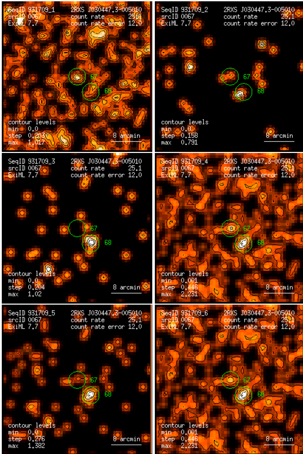
Figure 67: RASS 931709: detection 0067: band rate images, Gaussian filter: (1) PSPC channels 11 – 41, (2) 52 – 90, (3) 91 – 201, (4) 11 – 235, (5) 52 – 201, (6) 11 – 201. Broad band rates in counts/ks. Band rate contour levels in counts/ks/arcmin 2 .
