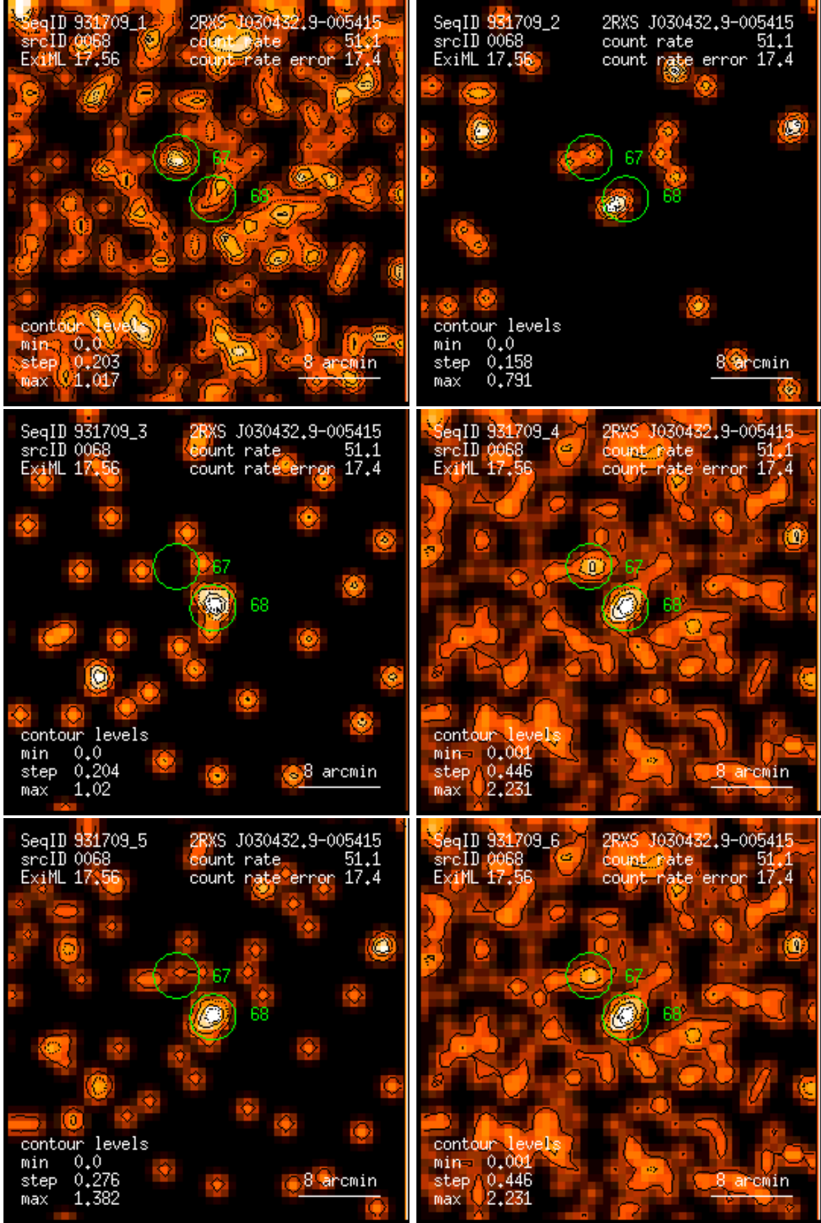
Figure 68: RASS 931709: detection 0068: band rate images, Gaussian filter: (1) PSPC channels 11 – 41, (2) 52 – 90, (3) 91 – 201, (4) 11 – 235, (5) 52 – 201, (6) 11 – 201. Broad band rates in counts/ks. Band rate contour levels in counts/ks/arcmin 2 .
