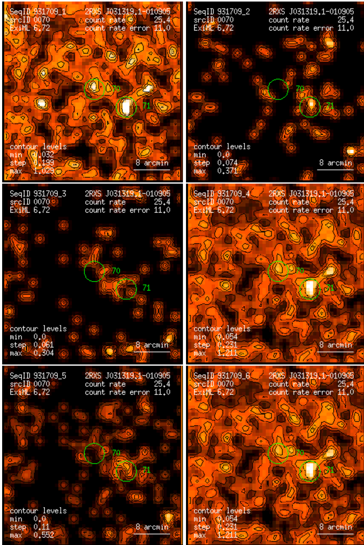
Figure 70: RASS 931709: detection 0070: band rate images, Gaussian filter: (1) PSPC channels 11 – 41, (2) 52 – 90, (3) 91 – 201, (4) 11 – 235, (5) 52 – 201, (6) 11 – 201. Broad band rates in counts/ks. Band rate contour levels in counts/ks/arcmin 2 .
