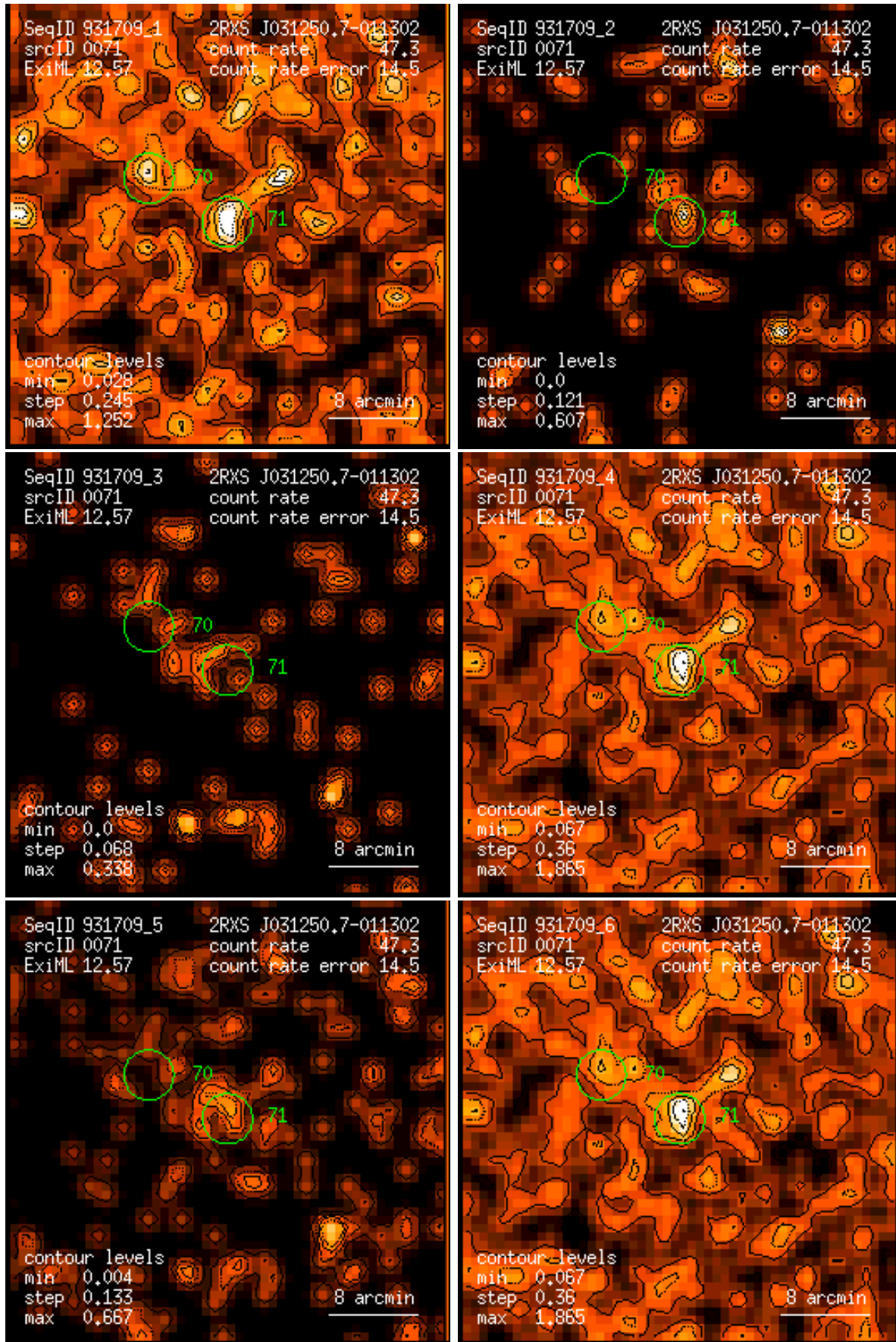
Figure 71: RASS 931709: detection 0071: band rate images, Gaussian filter: (1) PSPP channels 11 – 41, (2) 52 – 90, (3) 91 – 201, (4) 11 – 235, (5) 52 – 201, (6) 11 – 201. Broad band rates in counts/ks. Band rate contour levels in counts/ks/arcmin 2 .
