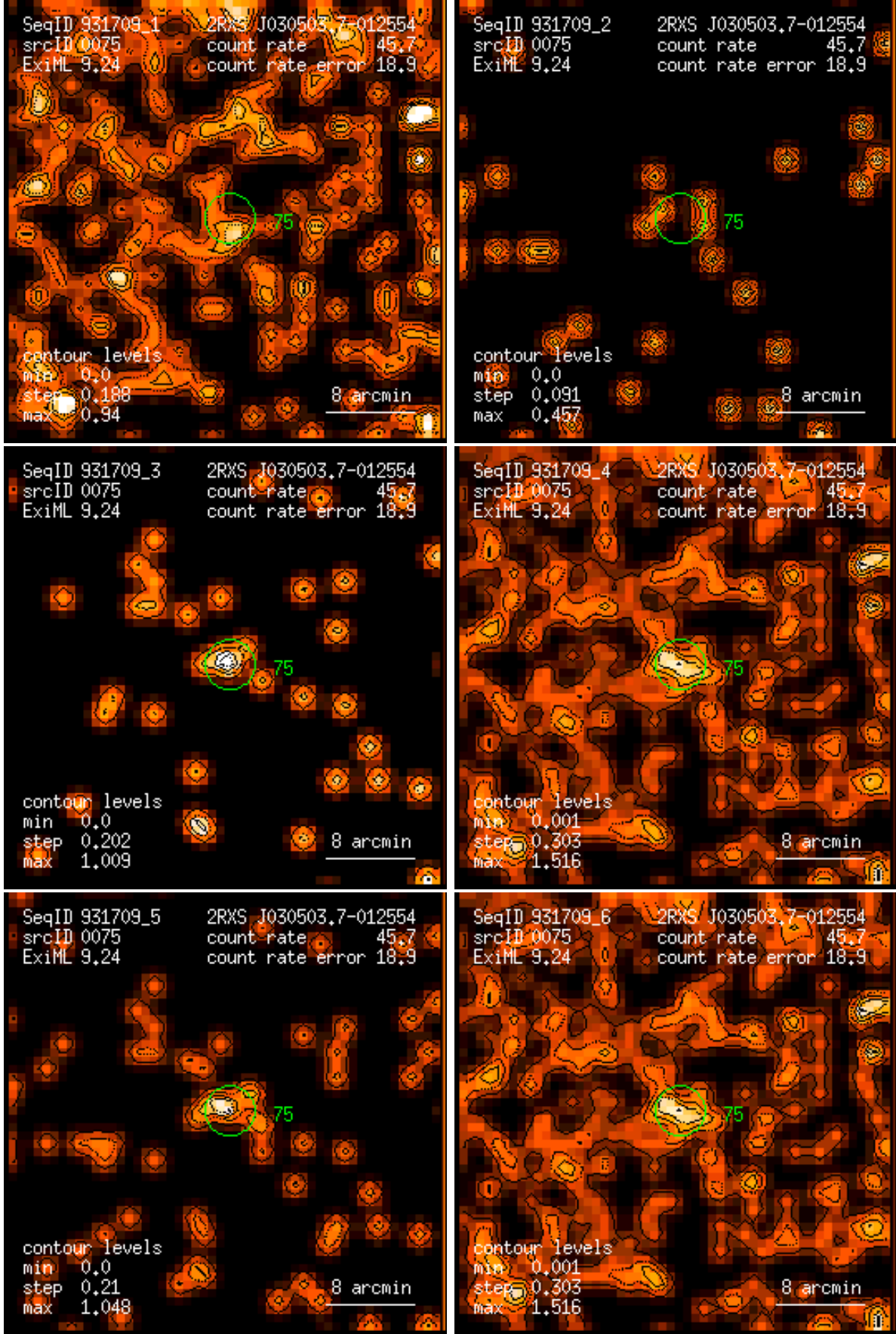
Figure 75: RASS 931709: detection 0075: band rate images, Gaussian filter: (1) PSPC channels 11 – 41, (2) 52 – 90, (3) 91 – 201, (4) 11 – 235, (5) 52 – 201, (6) 11 – 201. Broad band rates in counts/ks. Band rate contour levels in counts/ks/arcmin 2 .
