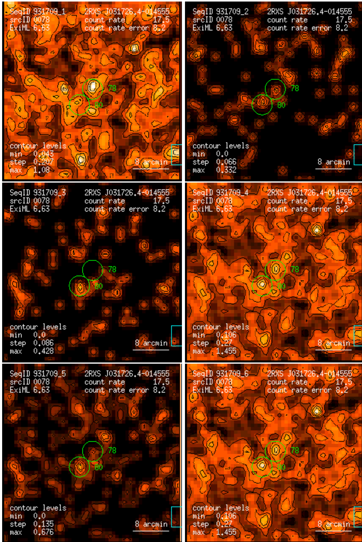
Figure 78: RASS 931709: detection 0078: band rate images, Gaussian filter: (1) PSPC channels 11 – 41, (2) 52 – 90, (3) 91 – 201, (4) 11 – 235, (5) 52 – 201, (6) 11 – 201. Broad band rates in counts/ks. Band rate contour levels in counts/ks/arcmin 2 .
