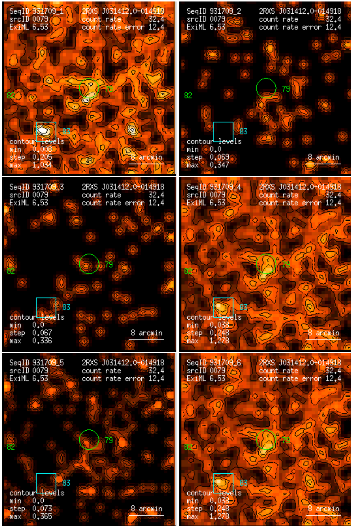
Figure 79: RASS 931709: detection 0079: band rate images, Gaussian filter: (1) PSPC channels 11 – 41, (2) 52 – 90, (3) 91 – 201, (4) 11 – 235, (5) 52 – 201, (6) 11 – 201. Broad band rates in counts/ks. Band rate contour levels in counts/ks/arcmin 2 .
