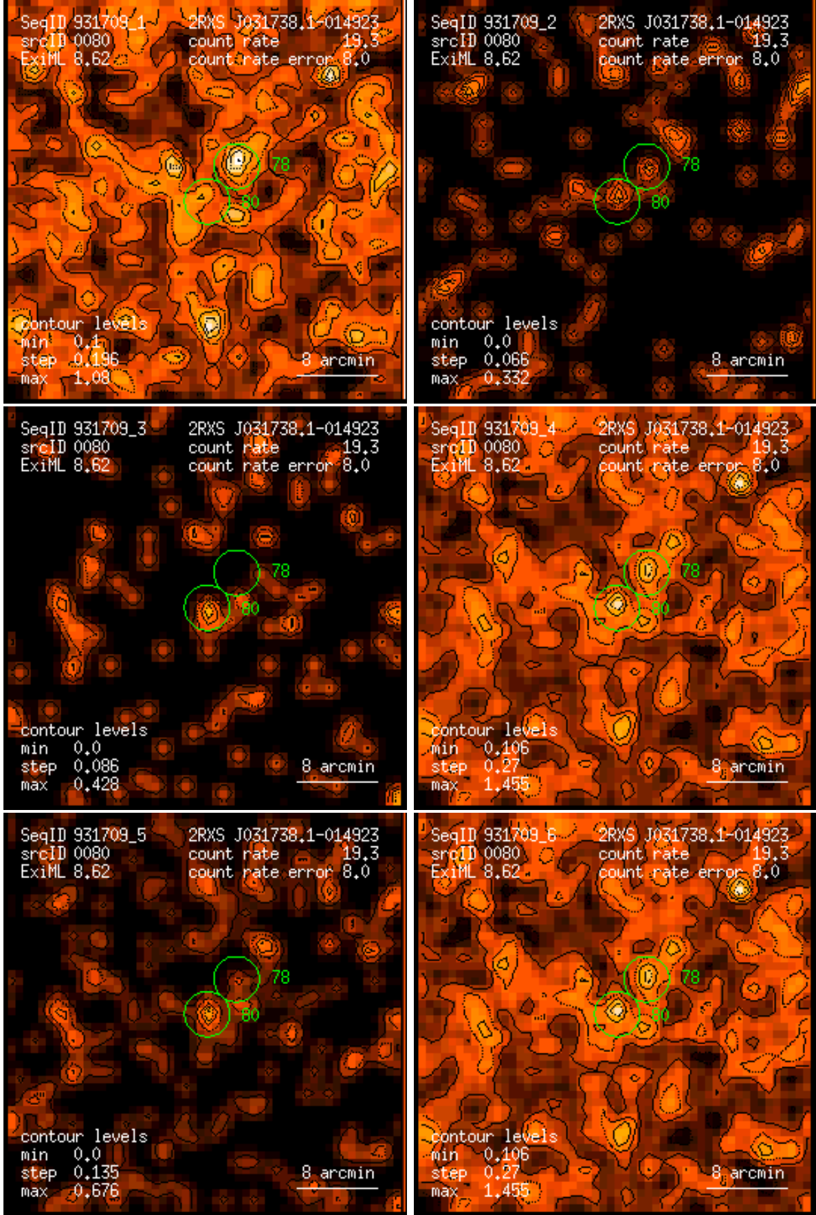
Figure 80: RASS 931709: detection 0080: band rate images, Gaussian filter: (1) PSPC channels 11 – 41, (2) 52 – 90, (3) 91 – 201, (4) 11 – 235, (5) 52 – 201, (6) 11 – 201. Broad band rates in counts/ks. Band rate contour levels in counts/ks/arcmin 2 .
