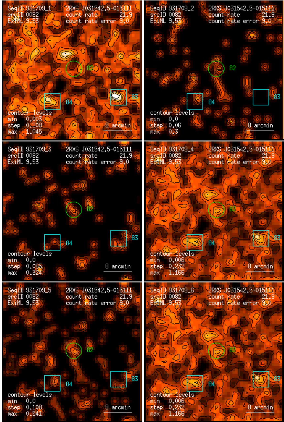
Figure 82: RASS 931709: detection 0082: band rate images, Gaussian filter: (1) PSPC channels 11 – 41, (2) 52 – 90, (3) 91 – 201, (4) 11 – 235, (5) 52 – 201, (6) 11 – 201. Broad band rates in counts/ks. Band rate contour levels in counts/ks/arcmin 2 .
