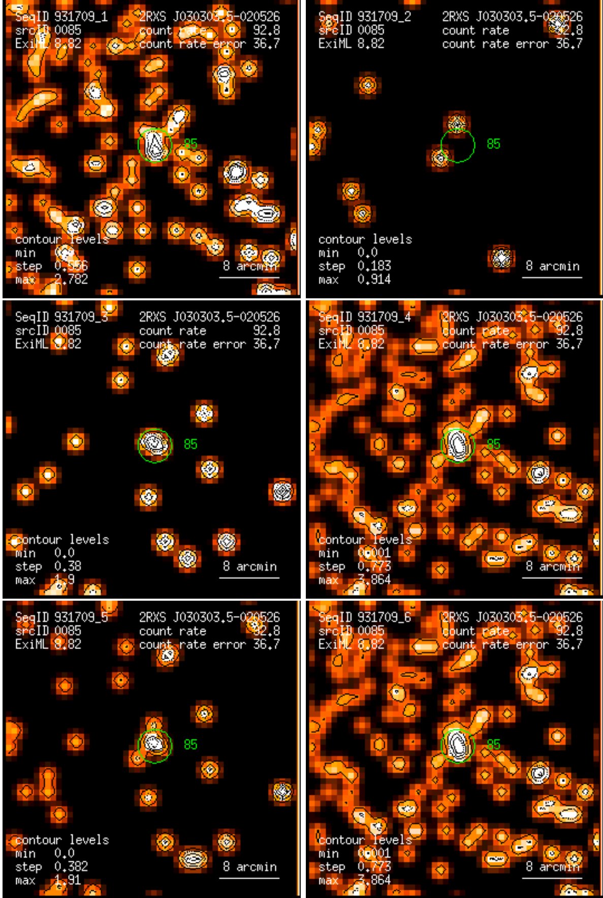
Figure 85: RASS 931709: detection 0085: band rate images, Gaussian filter: (1) PSPC channels 11 – 41, (2) 52 – 90, (3) 91 – 201, (4) 11 – 235, (5) 52 – 201, (6) 11 – 201. Broad band rates in counts/ks. Band rate contour levels in counts/ks/arcmin 2 .
