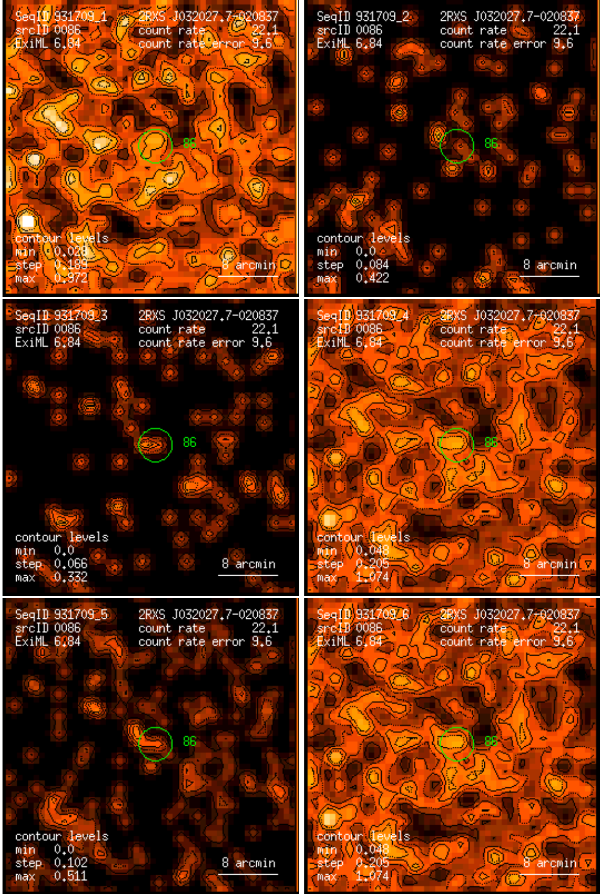
Figure 86: RASS 931709: detection 0086: band rate images, Gaussian filter: (1) PSPC channels 11 – 41, (2) 52 – 90, (3) 91 – 201, (4) 11 – 235, (5) 52 – 201, (6) 11 – 201. Broad band rates in counts/ks. Band rate contour levels in counts/ks/arcmin 2 .
