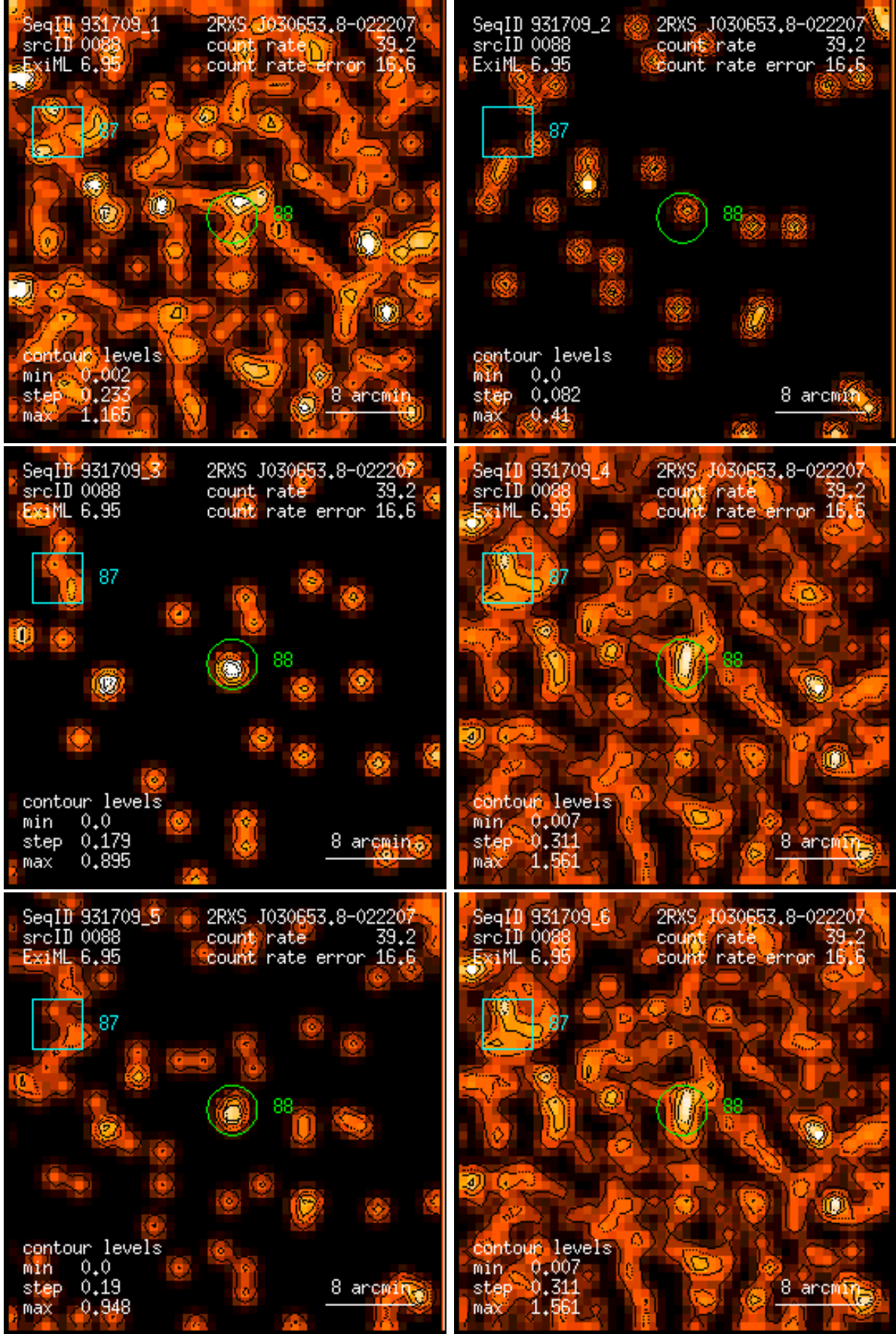
Figure 88: RASS 931709: detection 0088: band rate images, Gaussian filter: (1) PSPC channels 11 – 41, (2) 52 – 90, (3) 91 – 201, (4) 11 – 235, (5) 52 – 201, (6) 11 – 201. Broad band rates in counts/ks. Band rate contour levels in counts/ks/arcmin 2 .
