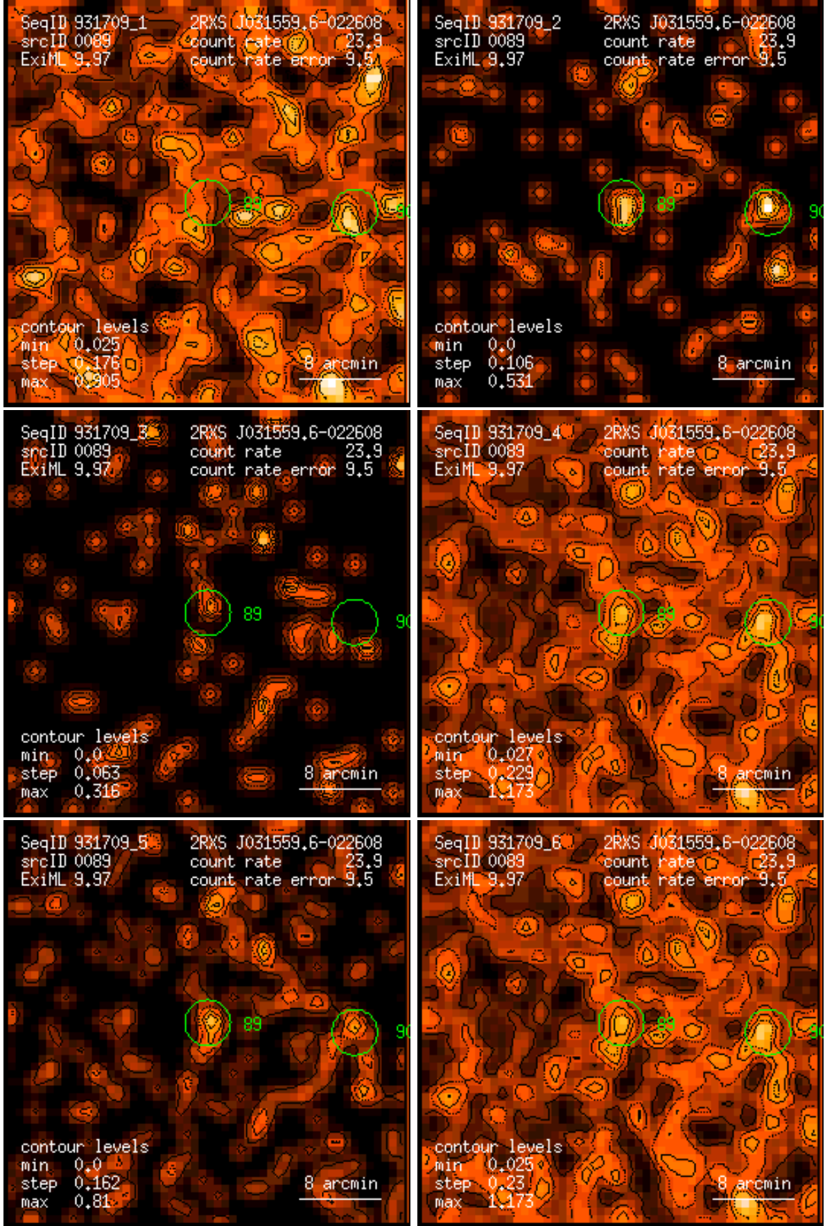
Figure 89: RASS 931709: detection 0089: band rate images, Gaussian filter: (1) PSPC channels 11 – 41, (2) 52 – 90, (3) 91 – 201, (4) 11 – 235, (5) 52 – 201, (6) 11 – 201. Broad band rates in counts/ks. Band rate contour levels in counts/ks/arcmin 2 .
