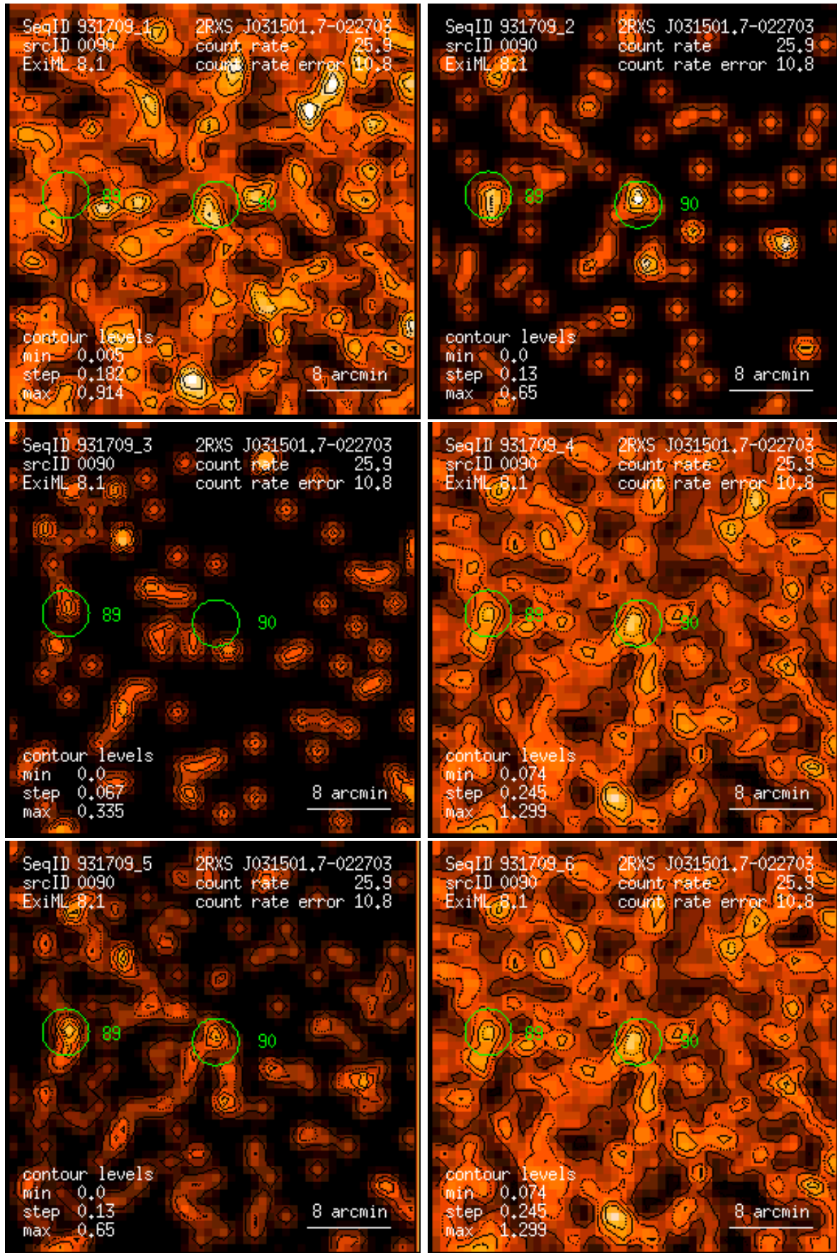
Figure 90: RASS 931709: detection 0090: band rate images, Gaussian filter: (1) PSPC channels 11 – 41, (2) 52 – 90, (3) 91 – 201, (4) 11 – 235, (5) 52 – 201, (6) 11 – 201. Broad band rates in counts/ks. Band rate contour levels in counts/ks/arcmin 2 .
