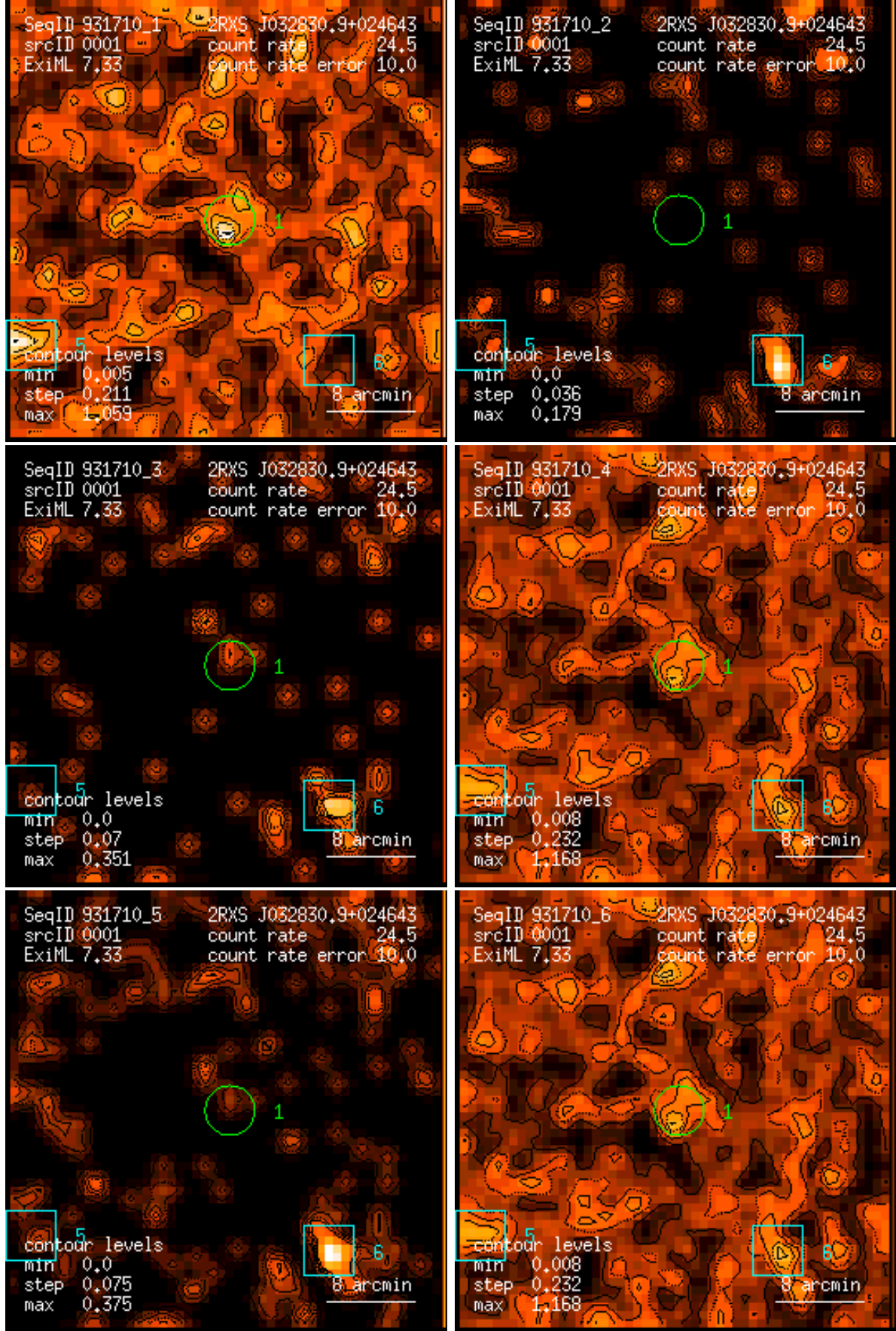
Figure 1: RASS 931710: detection 0001: band rate images, Gaussian filter: (1) PSPC channels 11 – 41, (2) 52 – 90, (3) 91 – 201, (4) 11 – 235, (5) 52 – 201, (6) 11 – 201. Broad band rates in counts/ks. Band rate contour levels in counts/ks/arcmin 2 .
