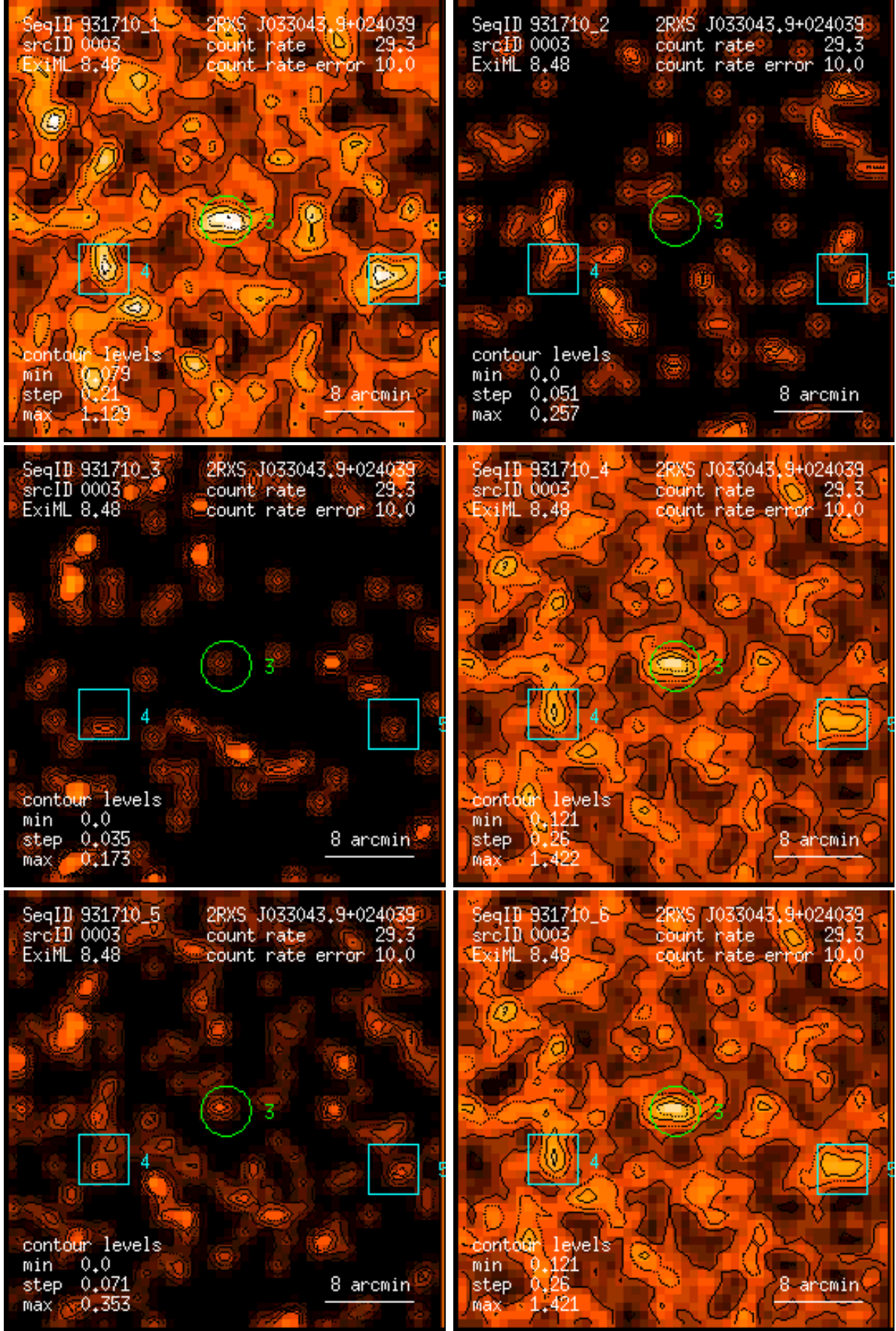
Figure 3: RASS 931710: detection 0003: band rate images, Gaussian filter: (1) PSPC channels 11 – 41, (2) 52 – 90, (3) 91 – 201, (4) 11 – 235, (5) 52 – 201, (6) 11 – 201. Broad band rates in counts/ks. Band rate contour levels in counts/ks/arcmin 2 .
