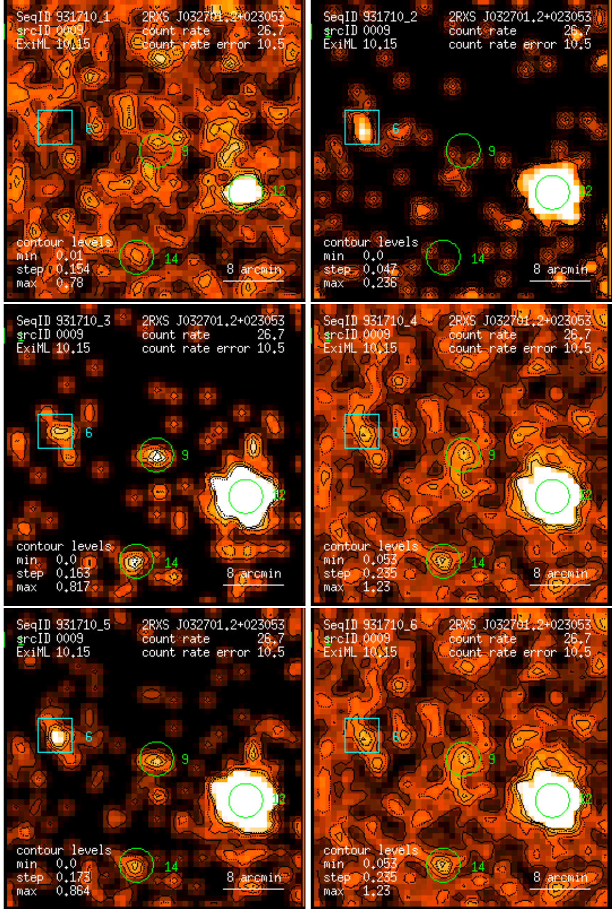
Figure 9: RASS 931710: detection 0009: band rate images, Gaussian filter: (1) PSPC channels 11 – 41, (2) 52 – 90, (3) 91 – 201, (4) 11 – 235, (5) 52 – 201, (6) 11 – 201. Broad band rates in counts/ks. Band rate contour levels in counts/ks/arcmin 2 .
