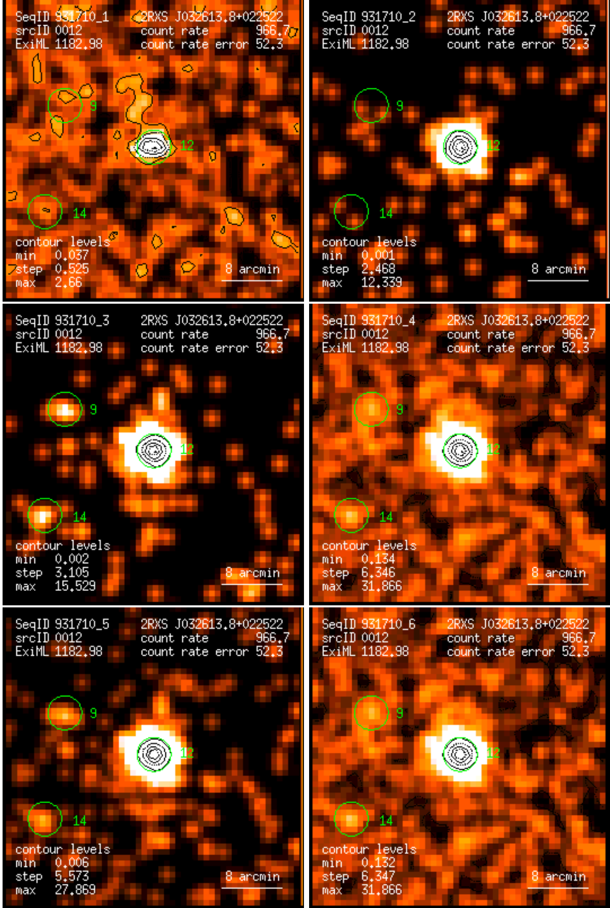
Figure 12: RASS 931710: detection 0012: band rate images, Gaussian filter: (1) PSPC channels 11 – 41, (2) 52 – 90, (3) 91 – 201, (4) 11 – 235, (5) 52 – 201, (6) 11 – 201. Broad band rates in counts/ks. Band rate contour levels in counts/ks/arcmin 2 .
