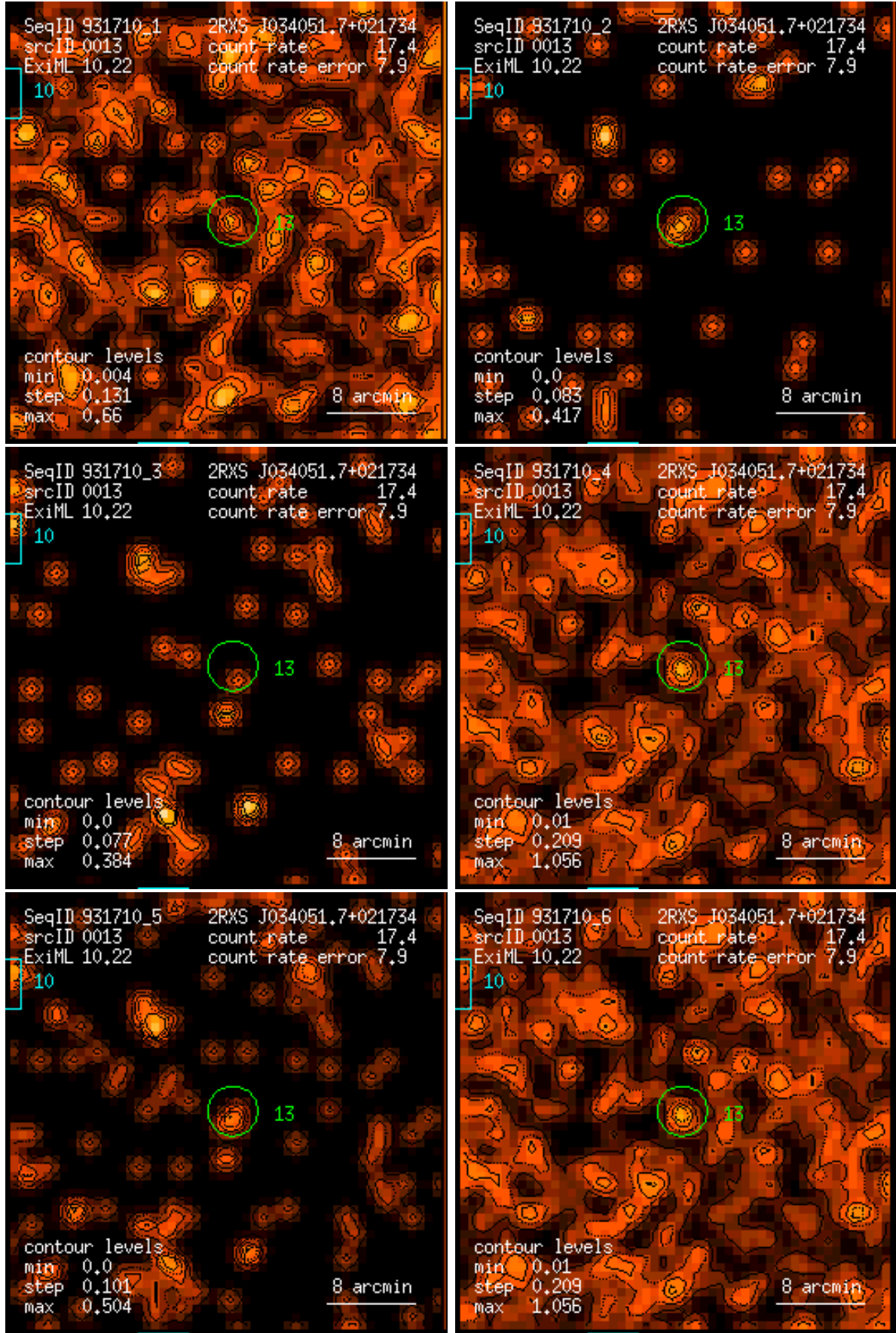
Figure 13: RASS 931710: detection 0013: band rate images, Gaussian filter: (1) PSPC channels 11 – 41, (2) 52 – 90, (3) 91 – 201, (4) 11 – 235, (5) 52 – 201, (6) 11 – 201. Broad band rates in counts/ks. Band rate contour levels in counts/ks/arcmin 2 .
