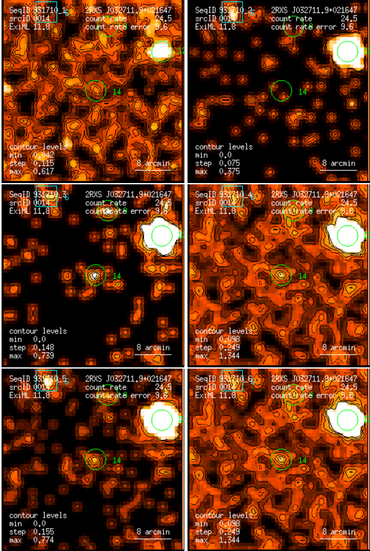
Figure 14: RASS 931710: detection 0014: band rate images, Gaussian filter: (1) PSPC channels 11 – 41, (2) 52 – 90, (3) 91 – 201, (4) 11 – 235, (5) 52 – 201, (6) 11 – 201. Broad band rates in counts/ks. Band rate contour levels in counts/ks/arcmin 2 .
