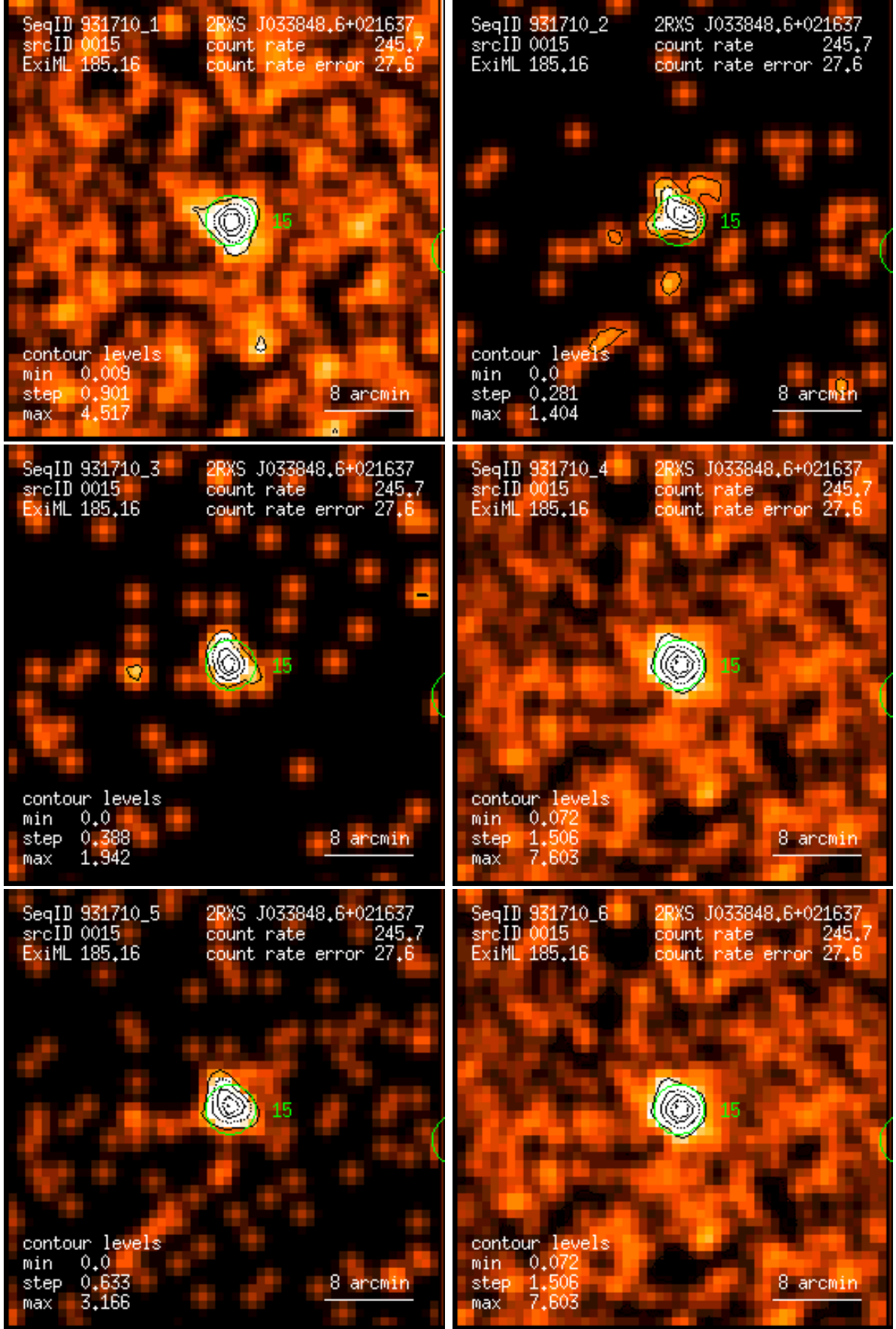
Figure 15: RASS 931710: detection 0015: band rate images, Gaussian filter: (1) PSPC channels 11 – 41, (2) 52 – 90, (3) 91 – 201, (4) 11 – 235, (5) 52 – 201, (6) 11 – 201. Broad band rates in counts/ks. Band rate contour levels in counts/ks/arcmin 2 .
