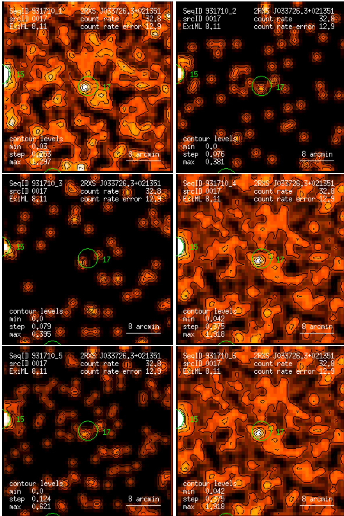
Figure 17: RASS 931710: detection 0017: band rate images, Gaussian filter: (1) PSPC channels 11 – 41, (2) 52 – 90, (3) 91 – 201, (4) 11 – 235, (5) 52 – 201, (6) 11 – 201. Broad band rates in counts/ks. Band rate contour levels in counts/ks/arcmin 2 .
