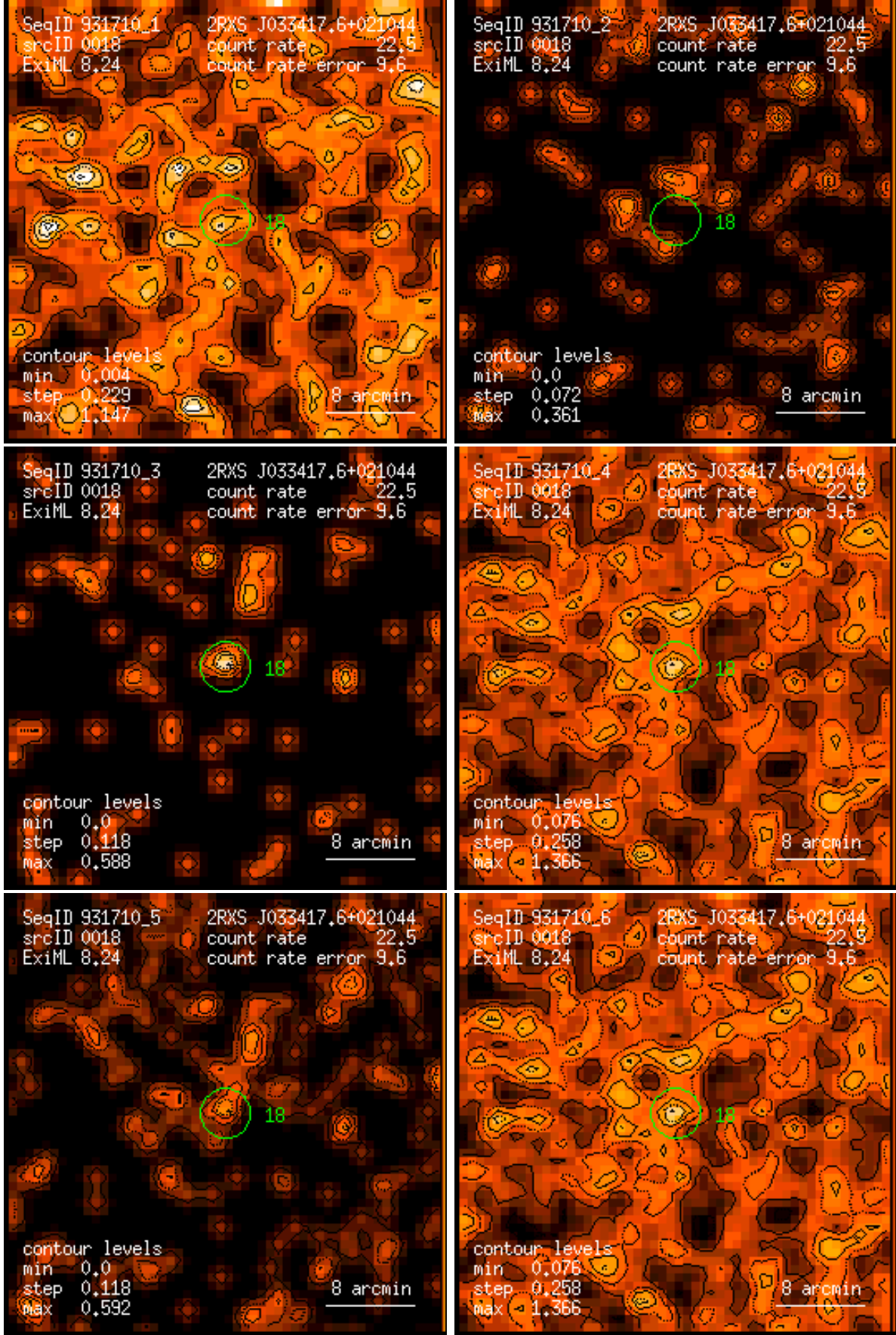
Figure 18: RASS 931710: detection 0018: band rate images, Gaussian filter: (1) PSPC channels 11 – 41, (2) 52 – 90, (3) 91 – 201, (4) 11 – 235, (5) 52 – 201, (6) 11 – 201. Broad band rates in counts/ks. Band rate contour levels in counts/ks/arcmin 2 .
