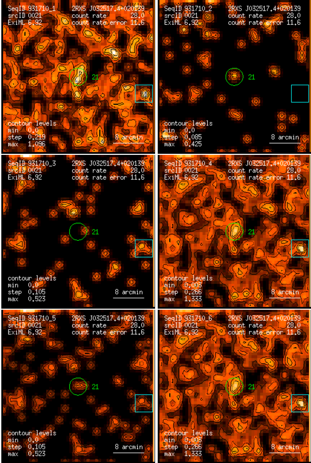
Figure 21: RASS 931710: detection 0021: band rate images, Gaussian filter: (1) PSPC channels 11 – 41, (2) 52 – 90, (3) 91 – 201, (4) 11 – 235, (5) 52 – 201, (6) 11 – 201. Broad band rates in counts/ks. Band rate contour levels in counts/ks/arcmin 2 .
