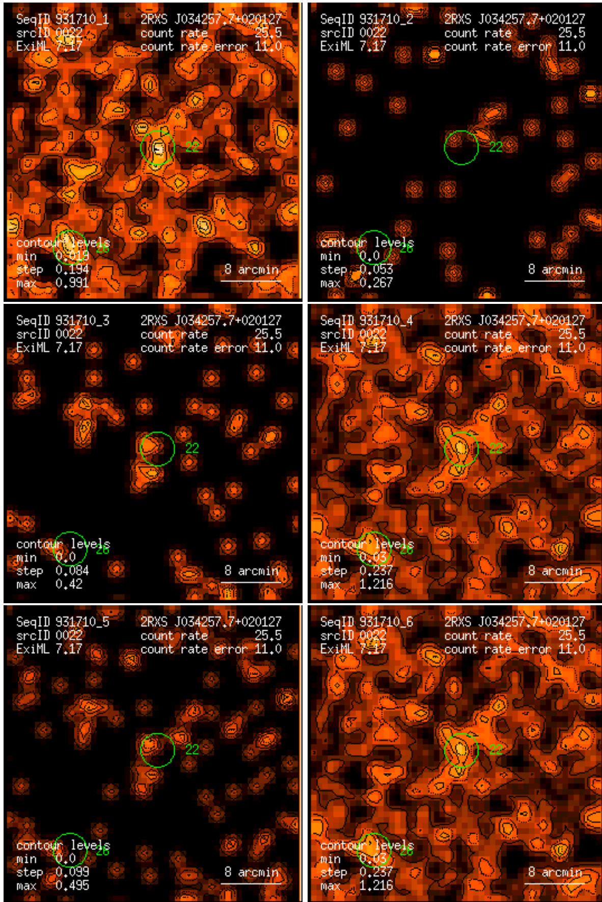
Figure 22: RASS 931710: detection 0022: band rate images, Gaussian filter: (1) PSPC channels 11 – 41, (2) 52 – 90, (3) 91 – 201, (4) 11 – 235, (5) 52 – 201, (6) 11 – 201. Broad band rates in counts/ks. Band rate contour levels in counts/ks/arcmin 2 .
