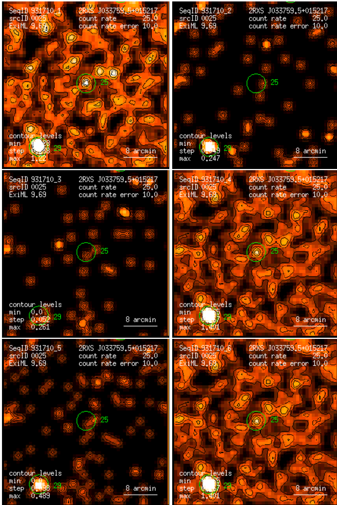
Figure 25: RASS 931710: detection 0025: band rate images, Gaussian filter: (1) PSPC channels 11 – 41, (2) 52 – 90, (3) 91 – 201, (4) 11 – 235, (5) 52 – 201, (6) 11 – 201. Broad band rates in counts/ks. Band rate contour levels in counts/ks/arcmin 2 .
