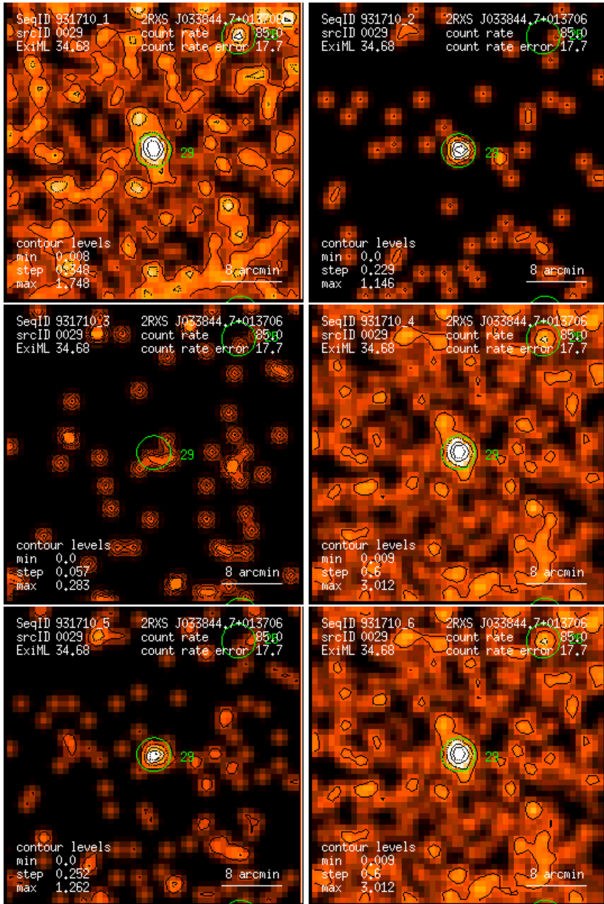
Figure 29: RASS 931710: detection 0029: band rate images, Gaussian filter: (1) PSPC channels 11 – 41, (2) 52 – 90, (3) 91 – 201, (4) 11 – 235, (5) 52 – 201, (6) 11 – 201. Broad band rates in counts/ks. Band rate contour levels in counts/ks/arcmin 2 .
