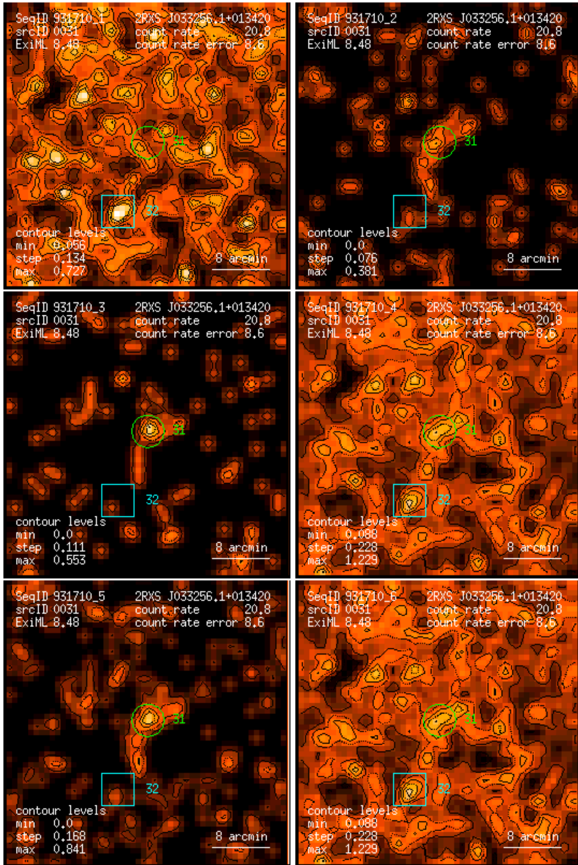
Figure 31: RASS 931710: detection 0031: band rate images, Gaussian filter: (1) PSPC channels 11 – 41, (2) 52 – 90, (3) 91 – 201, (4) 11 – 235, (5) 52 – 201, (6) 11 – 201. Broad band rates in counts/ks. Band rate contour levels in counts/ks/arcmin 2 .
