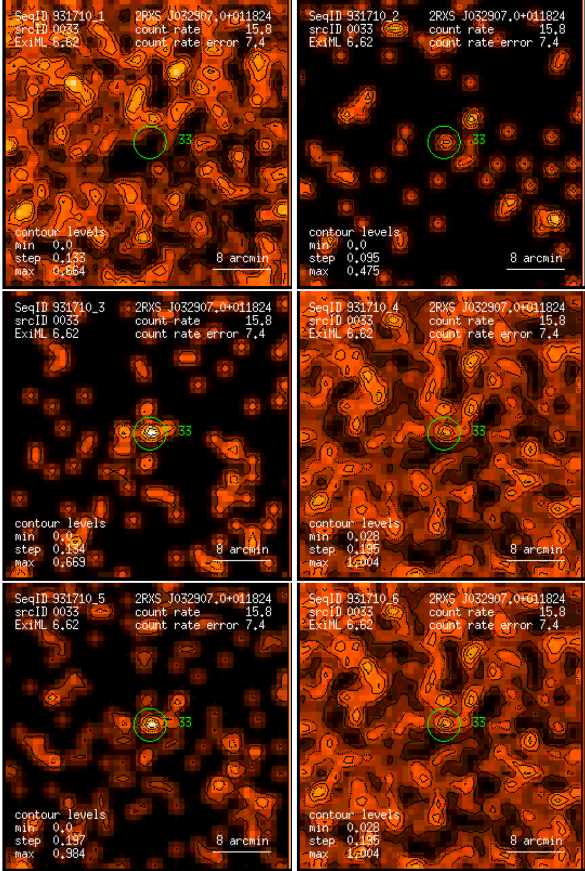
Figure 33: RASS 931710: detection 0033: band rate images, Gaussian filter: (1) PSPC channels 11 – 41, (2) 52 – 90, (3) 91 – 201, (4) 11 – 235, (5) 52 – 201, (6) 11 – 201. Broad band rates in counts/ks. Band rate contour levels in counts/ks/arcmin 2 .
