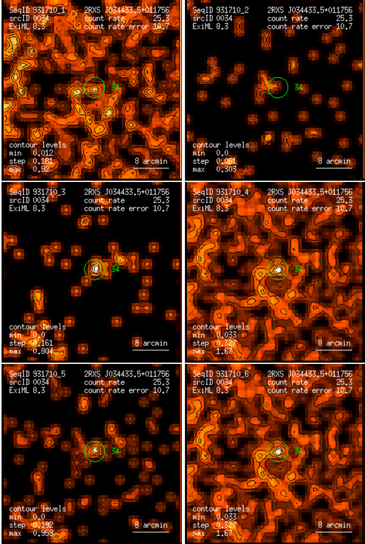
Figure 34: RASS 931710: detection 0034: band rate images, Gaussian filter: (1) PSPC channels 11 – 41, (2) 52 – 90, (3) 91 – 201, (4) 11 – 235, (5) 52 – 201, (6) 11 – 201. Broad band rates in counts/ks. Band rate contour levels in counts/ks/arcmin 2 .
