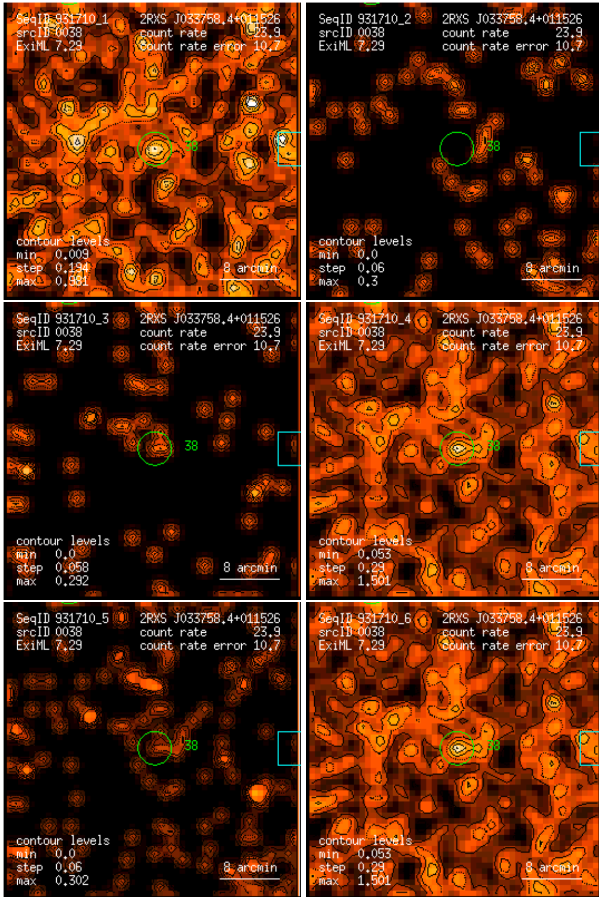
Figure 38: RASS 931710: detection 0038: band rate images, Gaussian filter: (1) PSPC channels 11 – 41, (2) 52 – 90, (3) 91 – 201, (4) 11 – 235, (5) 52 – 201, (6) 11 – 201. Broad band rates in counts/ks. Band rate contour levels in counts/ks/arcmin 2 .
