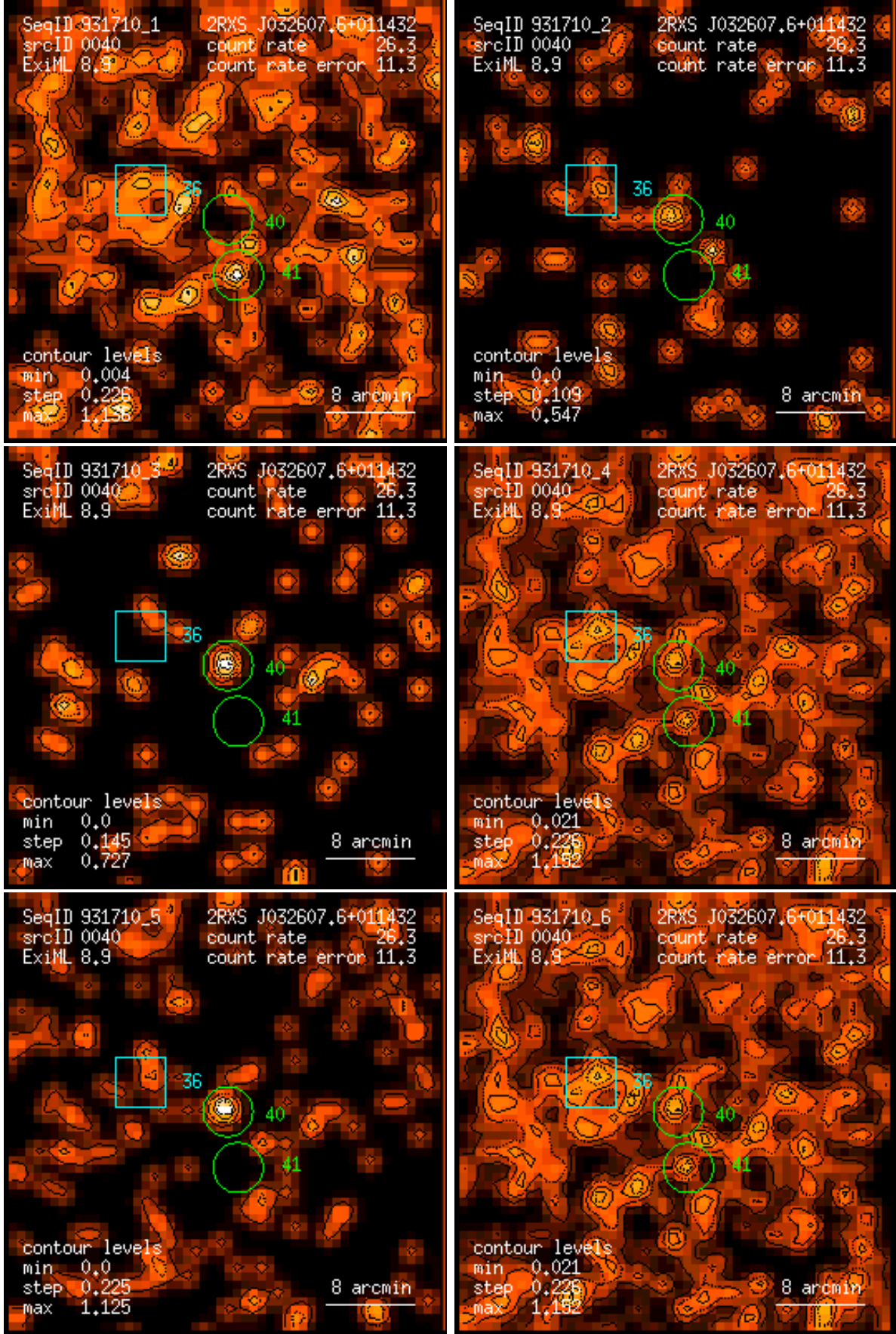
Figure 40: RASS 931710: detection 0040: band rate images, Gaussian filter: (1) PSPC channels 11 – 41, (2) 52 – 90, (3) 91 – 201, (4) 11 – 235, (5) 52 – 201, (6) 11 – 201. Broad band rates in counts/ks. Band rate contour levels in counts/ks/arcmin 2 .
