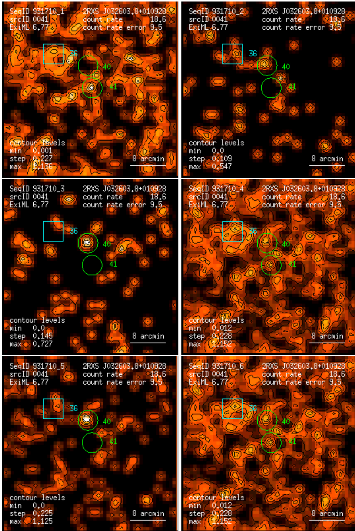
Figure 41: RASS 931710: detection 0041: band rate images, Gaussian filter: (1) PSPC channels 11 – 41, (2) 52 – 90, (3) 91 – 201, (4) 11 – 235, (5) 52 – 201, (6) 11 – 201. Broad band rates in counts/ks. Band rate contour levels in counts/ks/arcmin 2 .
