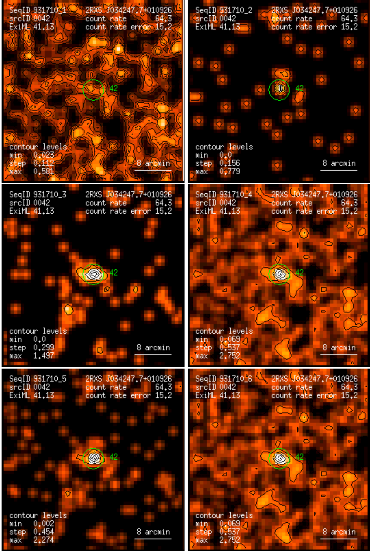
Figure 42: RASS 931710: detection 0042: band rate images, Gaussian filter: (1) PSPC channels 11 – 41, (2) 52 – 90, (3) 91 – 201, (4) 11 – 235, (5) 52 – 201, (6) 11 – 201. Broad band rates in counts/ks. Band rate contour levels in counts/ks/arcmin 2 .
