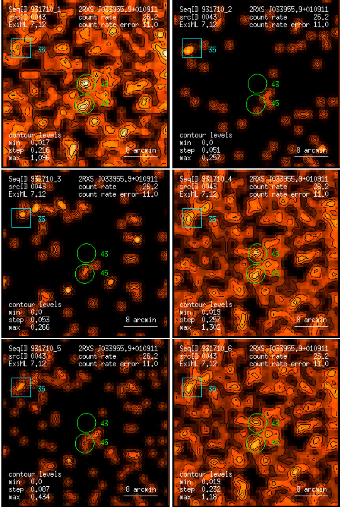
Figure 43: RASS 931710: detection 0043: band rate images, Gaussian filter: (1) PSPC channels 11 – 41, (2) 52 – 90, (3) 91 – 201, (4) 11 – 235, (5) 52 – 201, (6) 11 – 201. Broad band rates in counts/ks. Band rate contour levels in counts/ks/arcmin 2 .
