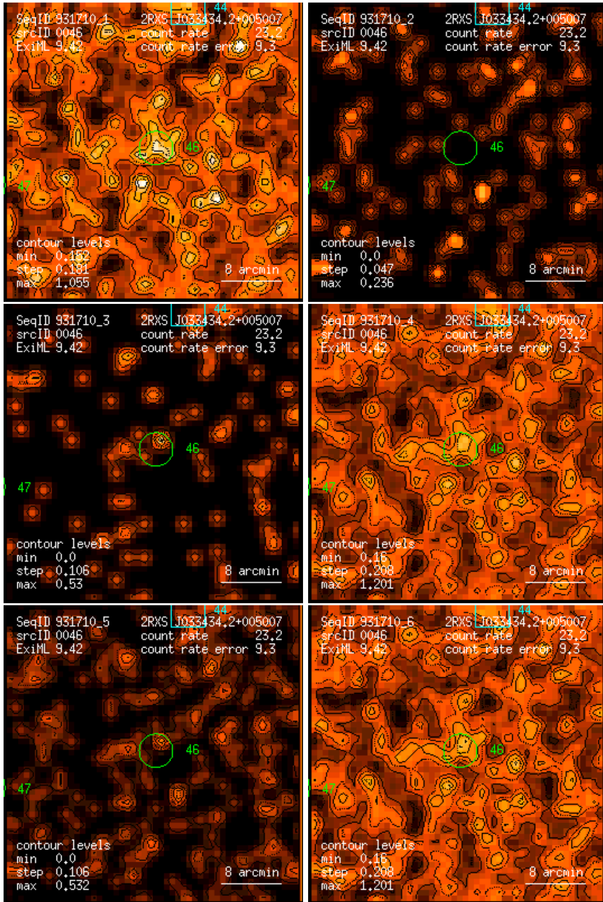
Figure 46: RASS 931710: detection 0046: band rate images, Gaussian filter: (1) PSPC channels 11 – 41, (2) 52 – 90, (3) 91 – 201, (4) 11 – 235, (5) 52 – 201, (6) 11 – 201. Broad band rates in counts/ks. Band rate contour levels in counts/ks/arcmin 2 .
